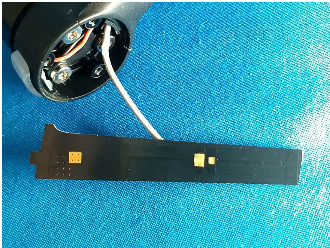
SRD Antenna 0
