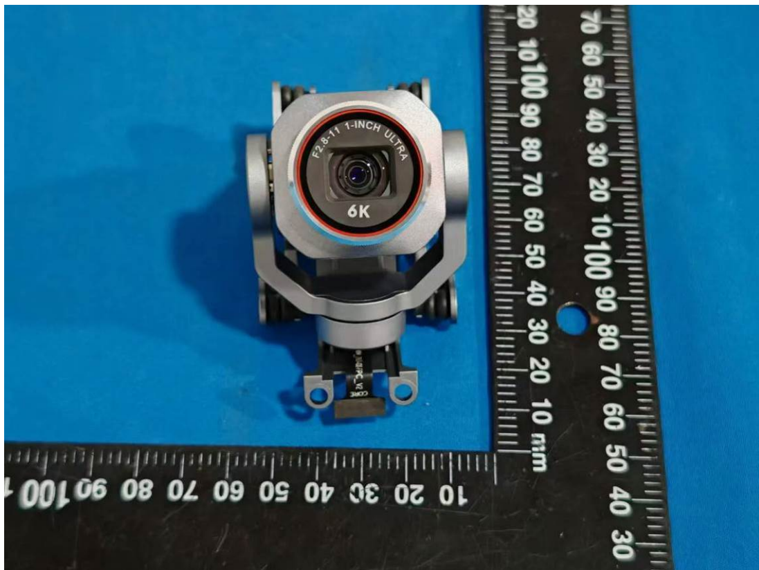
Gimbal camera 1#(Camera for EVO Lite+ and EVO Lite 6K Enterprise)
