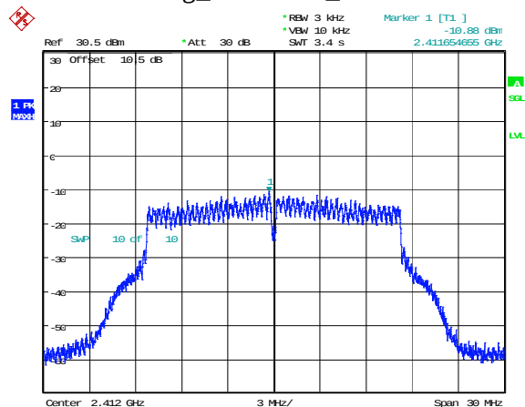
802.11g_2412MHz_Chain 0
