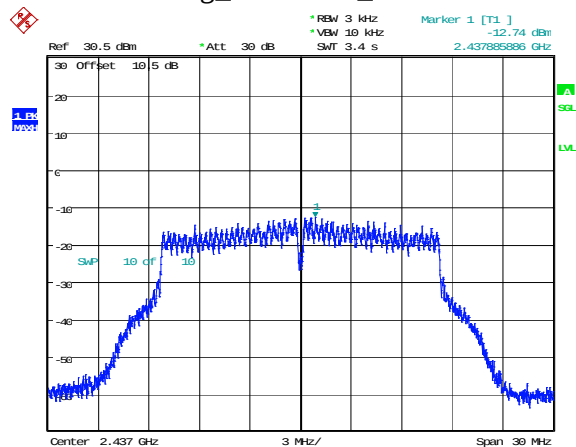
802.11g_2437MHz_Chain 1
