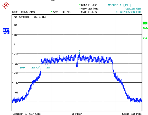
802.11g_2437MHz_Chain 0
