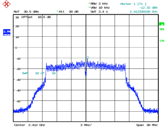
802.11g_2412MHz_Chain 1
