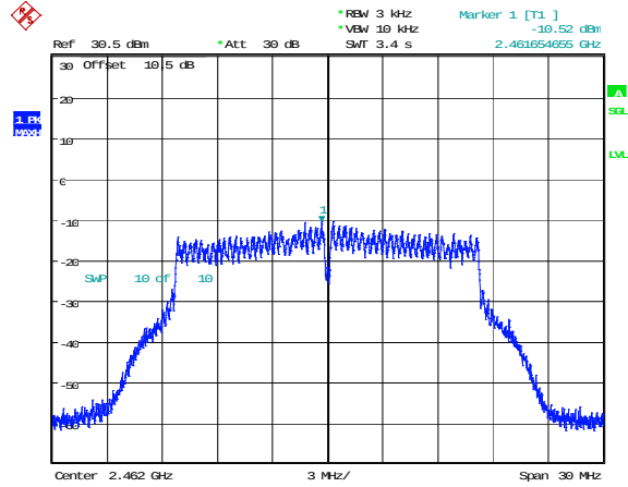
802.11g_2462MHz_Chain 0
