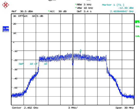
802.11g_2462MHz_Chain 1
