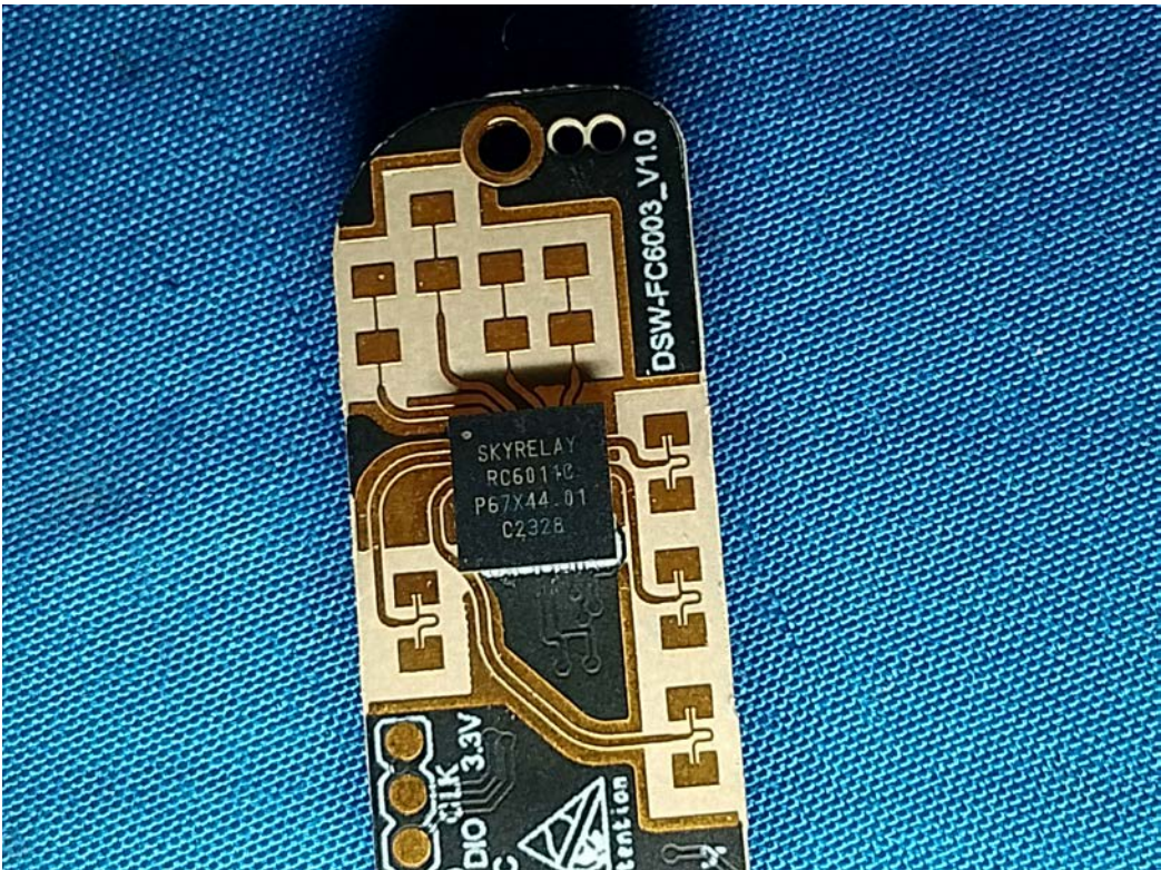
Rear Radar Antenna
