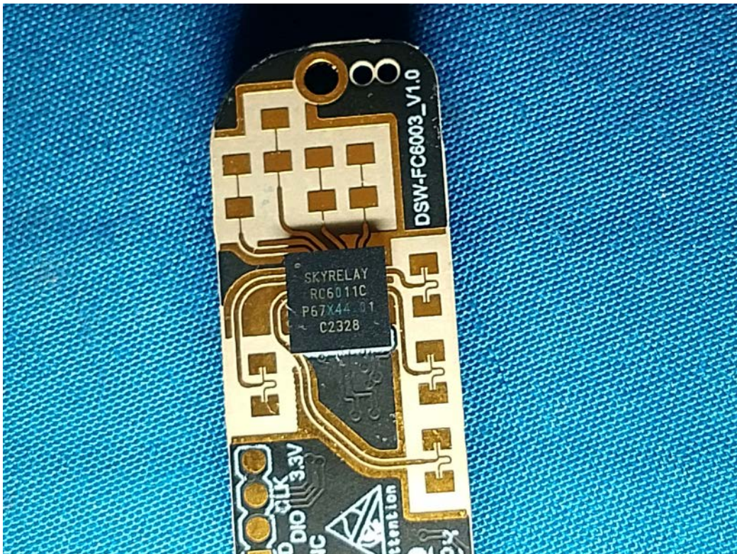
Front Radar Antenna
