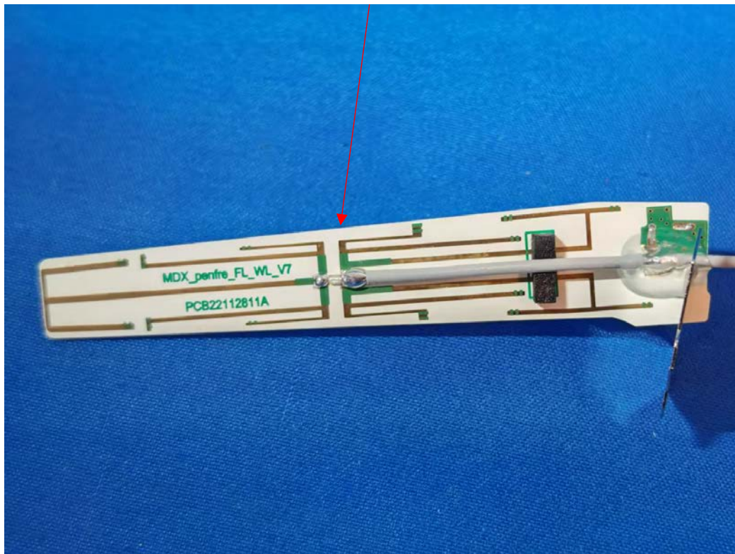
SRD ANT 3(Chain 1)
