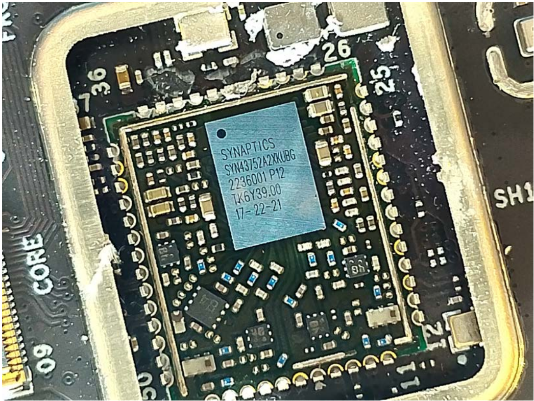
Chip
