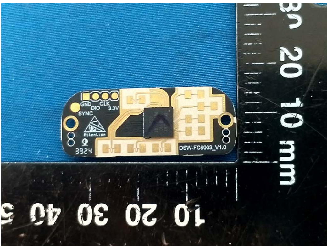
Bottom Radar
