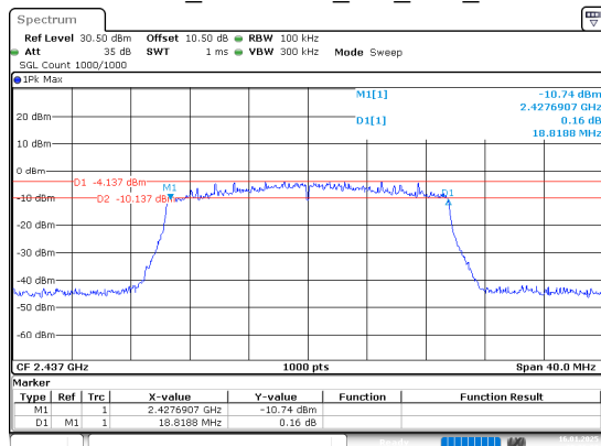
802.11ax20_2437MHz_RU_Full_Chain 0
