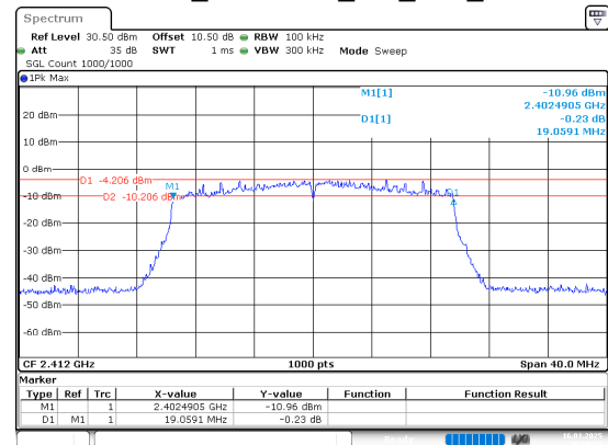
802.11ax20_2412MHz_RU_Full_Chain 0
