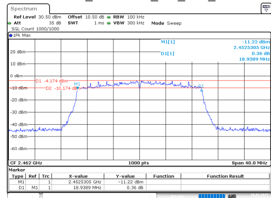
802.11ax20_2462MHz_RU_Full_Chain 0
