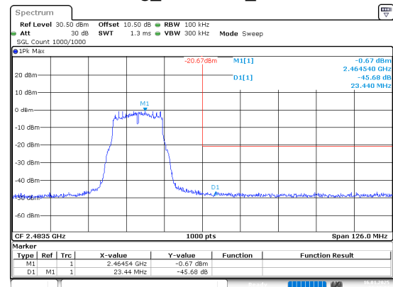
802.11g_2462MHz_Chain 0
