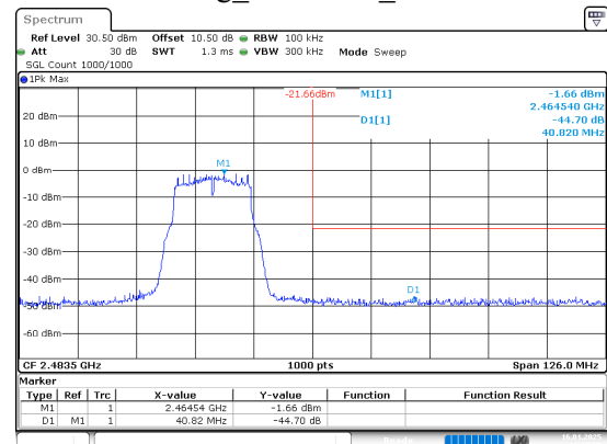
802.11g_2462MHz_Chain 1
