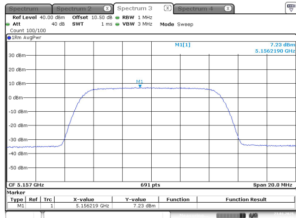
10M_5157MHz
