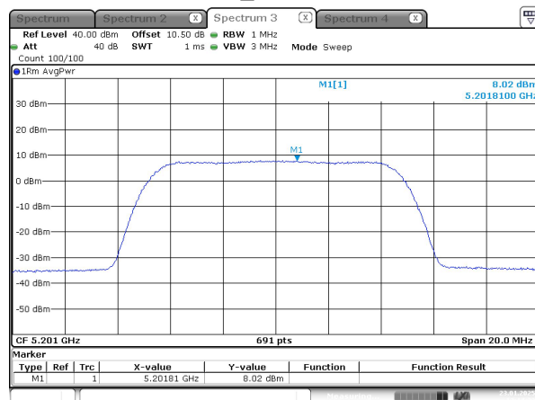
10M_5201MHz
