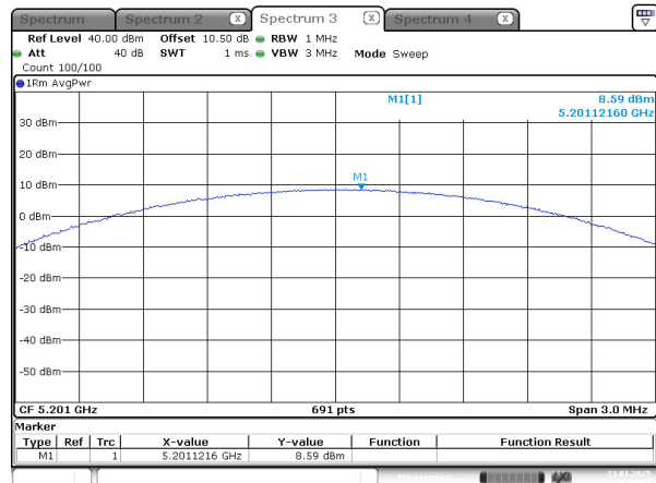
1.4M_5201MHz
