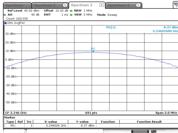
1.4M_5246MHz
