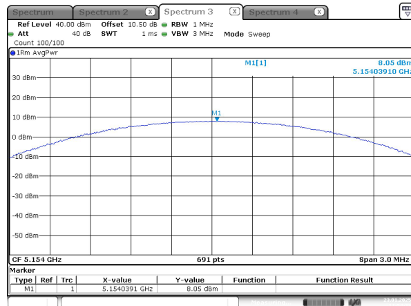
1.4M_5154MHz
