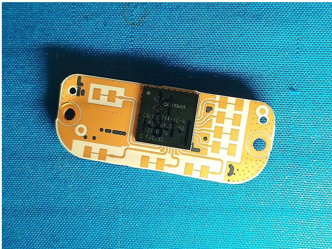
Chip+ANT
