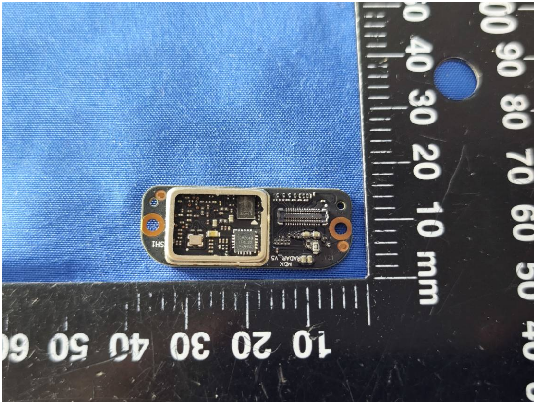
Rear radar
