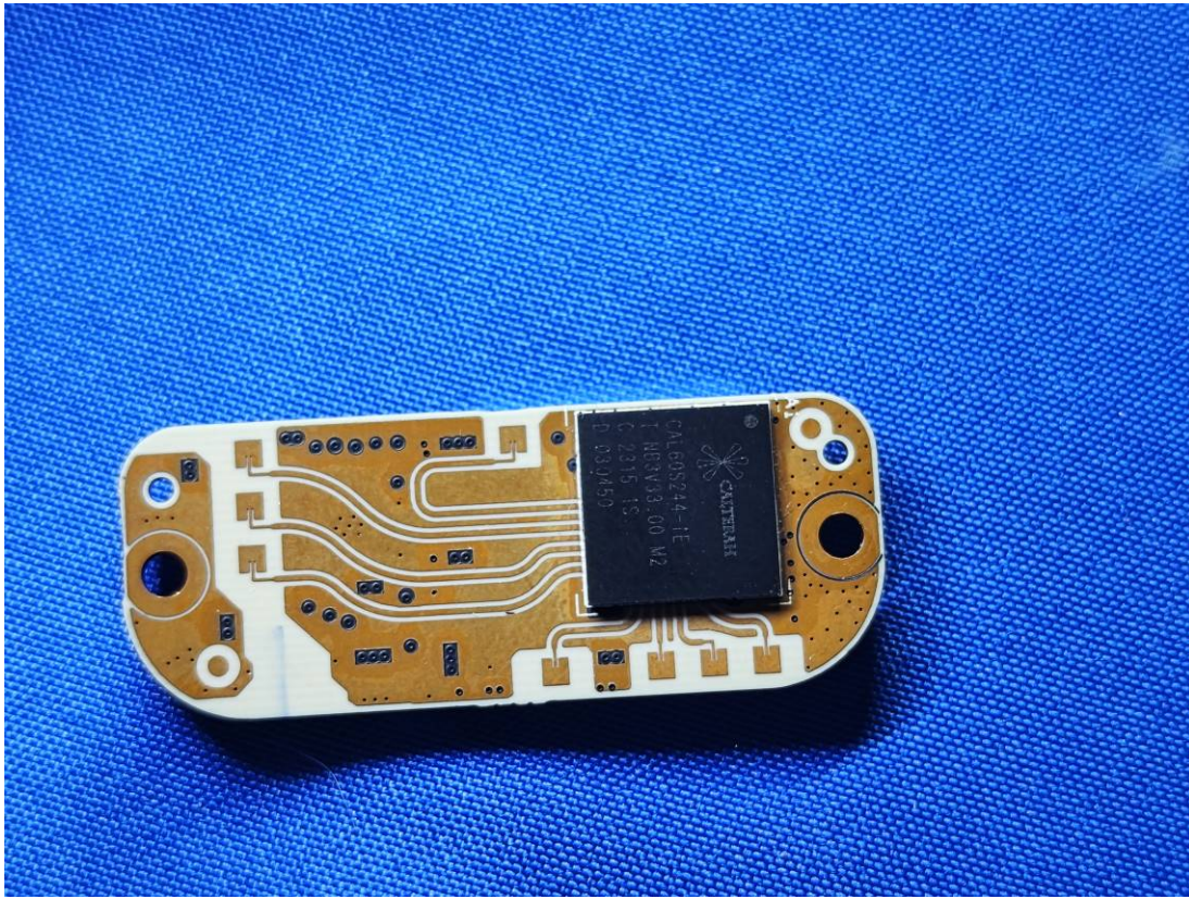
Top radar
