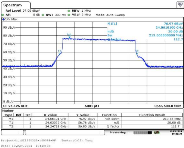
20 dB Bandwidth
