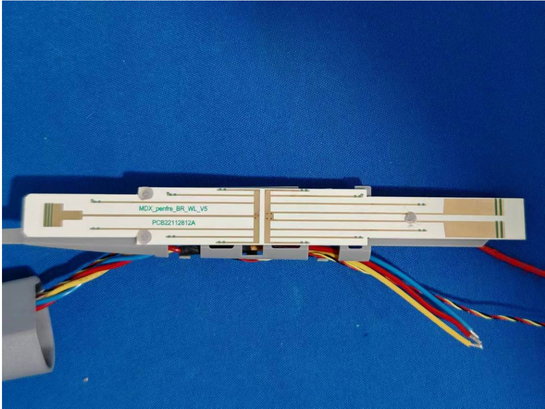
SRD Antenna 3(Back Right)
