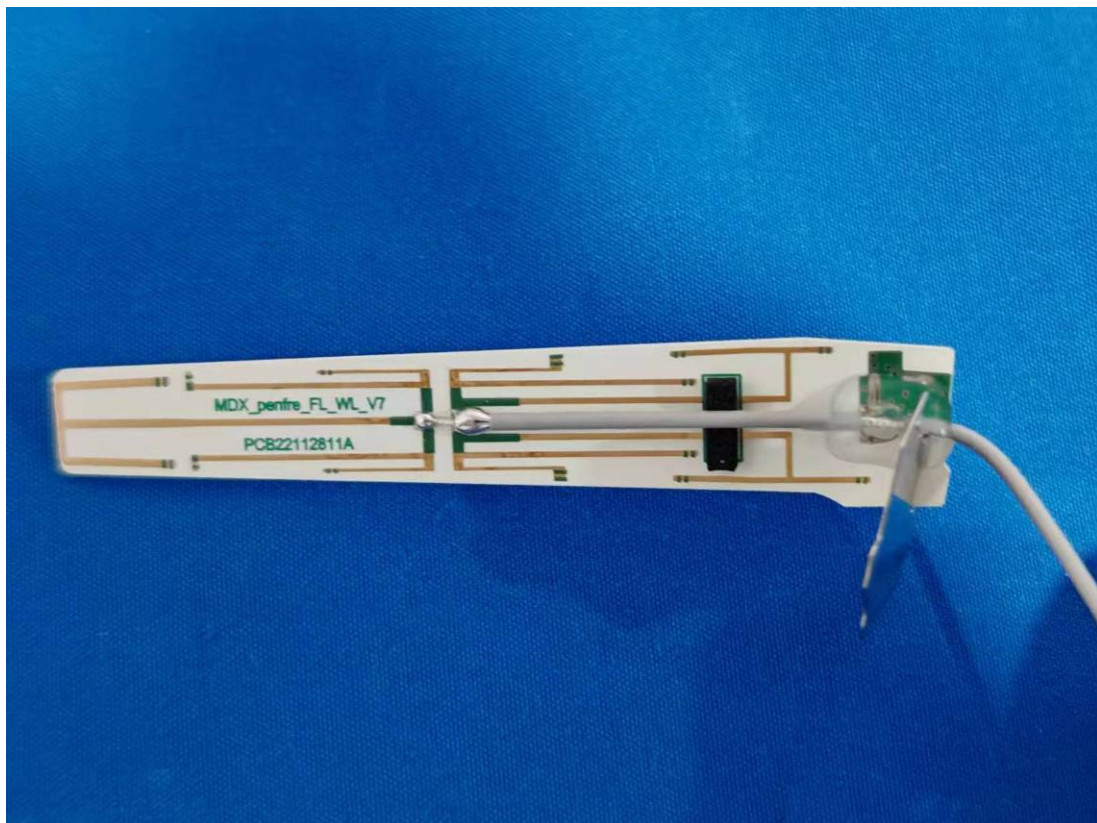
SRD Antenna 2(Front Left)
