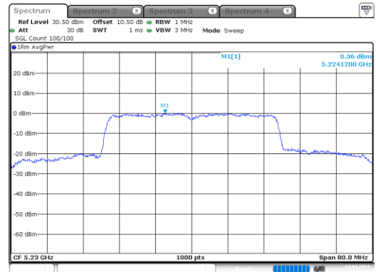
ax40_5230MHz_RU_Full_Chain 1
