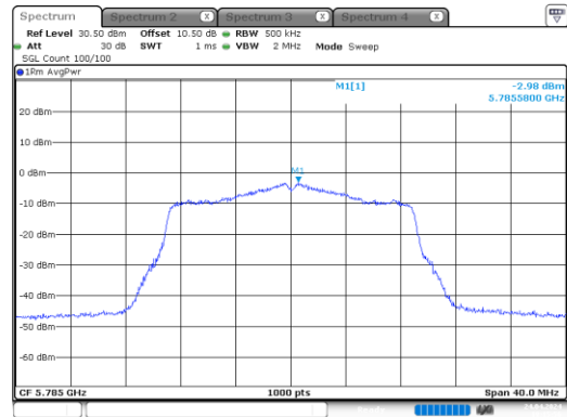
n20_5785MHz_Chain 1
