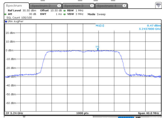
ax20_5240MHz_RU_Full_Chain 1
