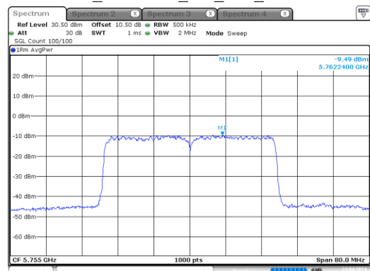
ax40_5755MHz_RU_Full_Chain 1
