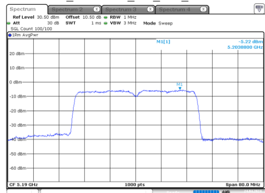
ax40_5190MHz_RU_Full_Chain 1
