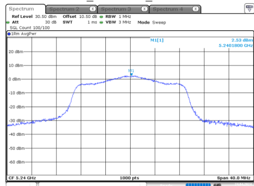
n20_5240MHz_Chain 1
