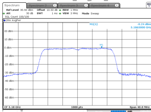
ax20_5180MHz_RU_Full_Chain 0
