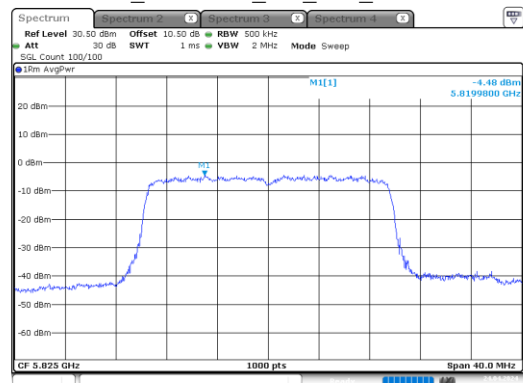
ax20_5825MHz_RU_Full_Chain 1
