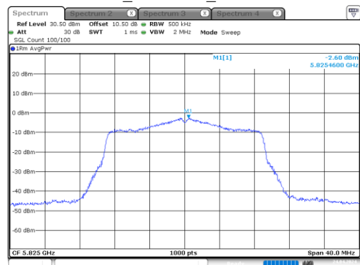
n20_5825MHz_Chain 1
