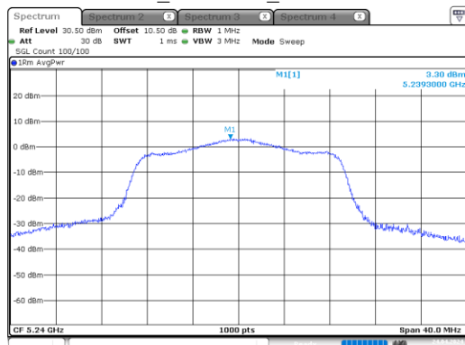
n20_5240MHz_Chain 0
