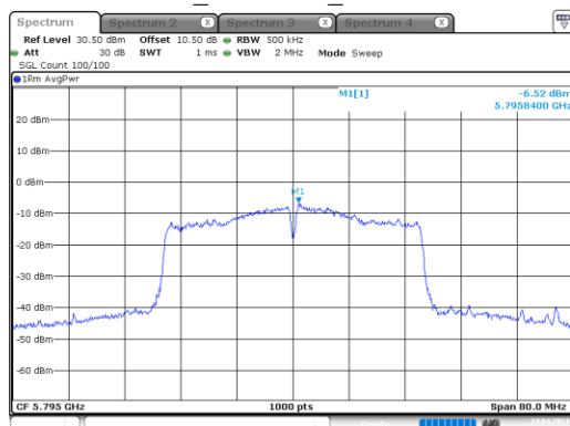
n40_5795MHz_Chain 0
