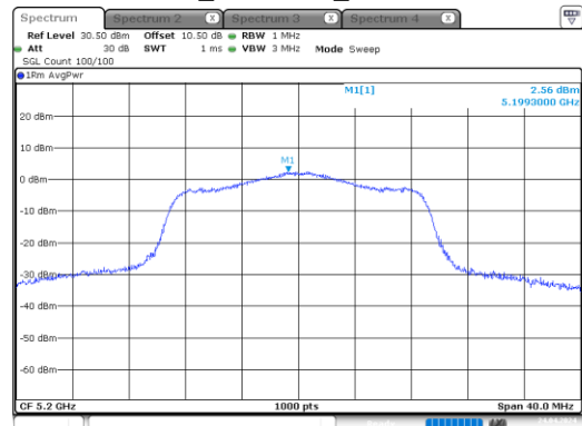
n20_5200MHz_Chain 1
