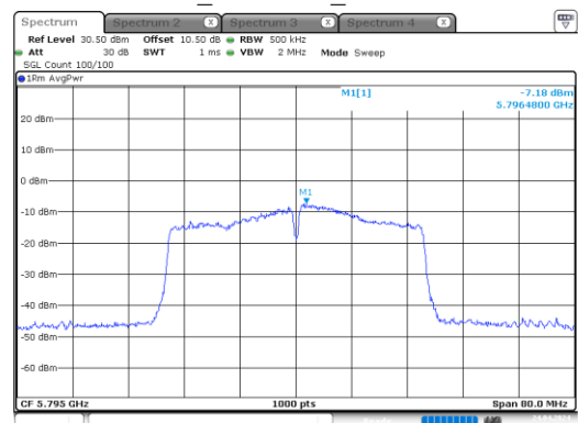
n40_5795MHz_Chain 1
