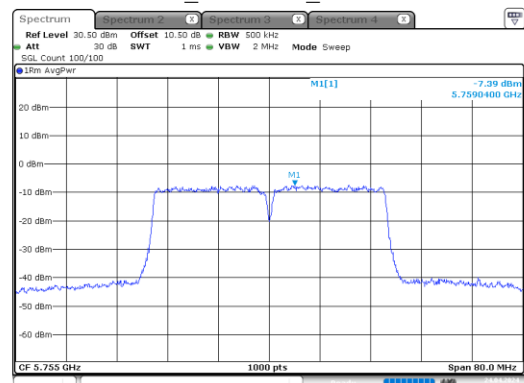
ac40_5755MHz_Chain 1
