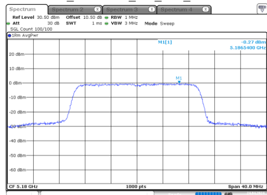
ax20_5180MHz_RU_Full_Chain 1
