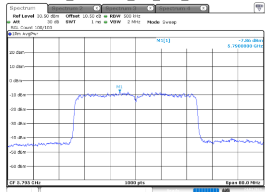
ax40_5795MHz_RU_Full_Chain 1
