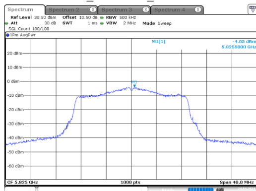
n20_5825MHz_Chain 0
