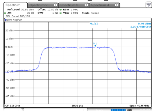
ax20_5200MHz_RU_Full_Chain 1
