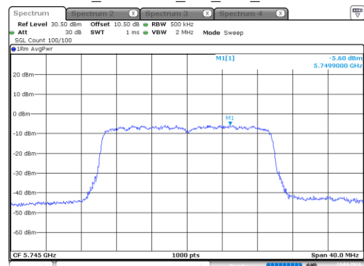
ax20_5745MHz_RU_Full_Chain 1
