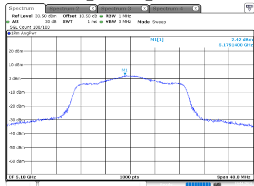
n20_5180MHz_Chain 1
