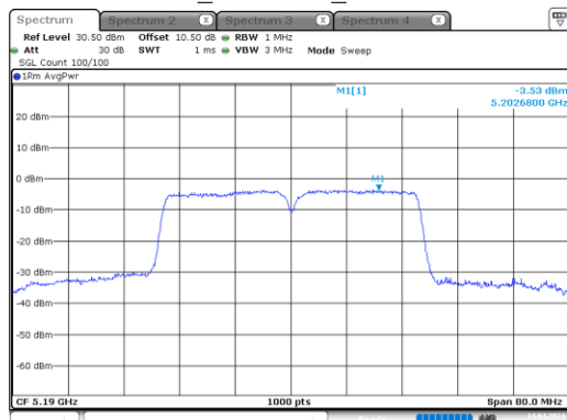
ac40_5190MHz_Chain 0
