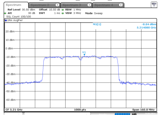
ax80_5210MHz_RU_Full_Chain 1
