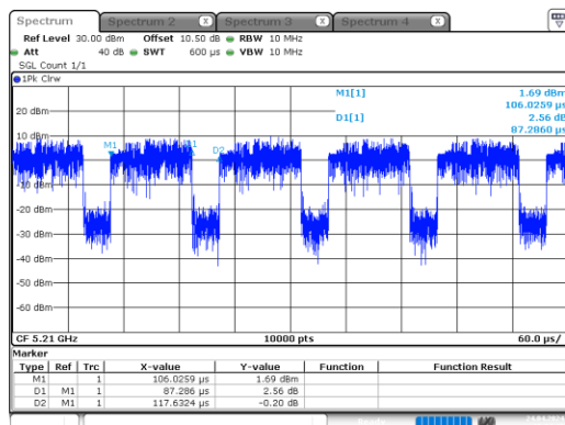
ax80_5210MHz_RU_Full_Chain 0
