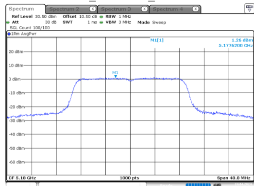
ac20_5180MHz_Chain 1
