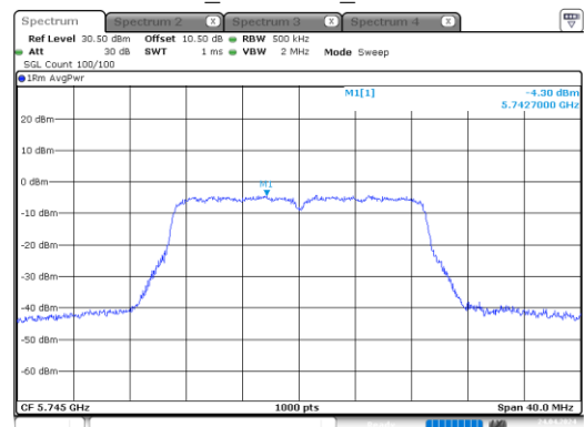
ac20_5745MHz_Chain 1
