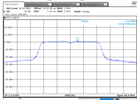
ac20_5240MHz_Chain 1
