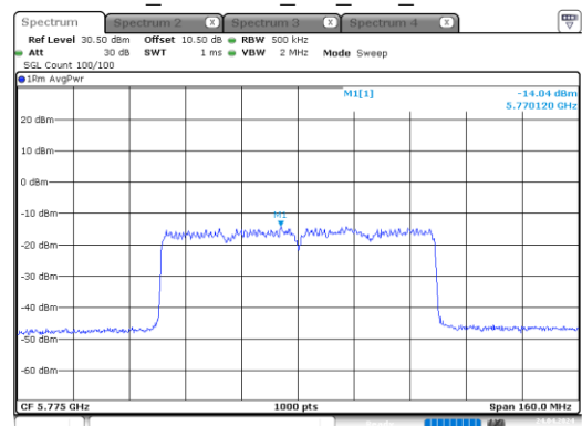
ax80_5775MHz_RU_Full_Chain 1
