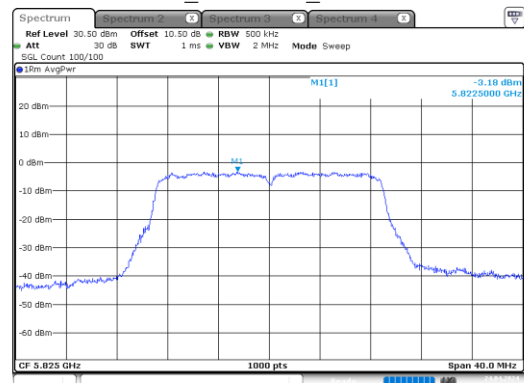
ac20_5825MHz_Chain 1
