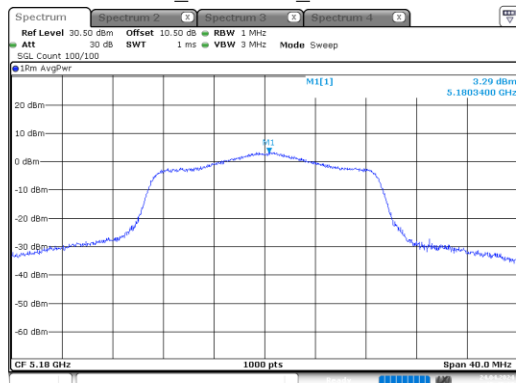
n20_5180MHz_Chain 0
