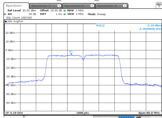
ac40_5190MHz_Chain 1
