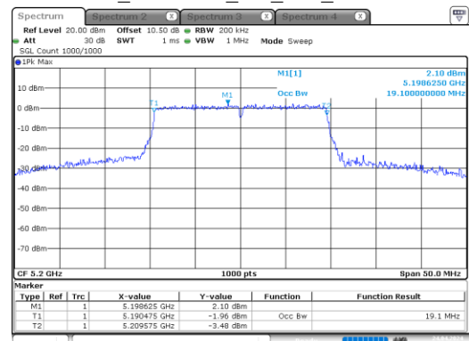
ax20_5200MHz_RU_Full_Chain 0
