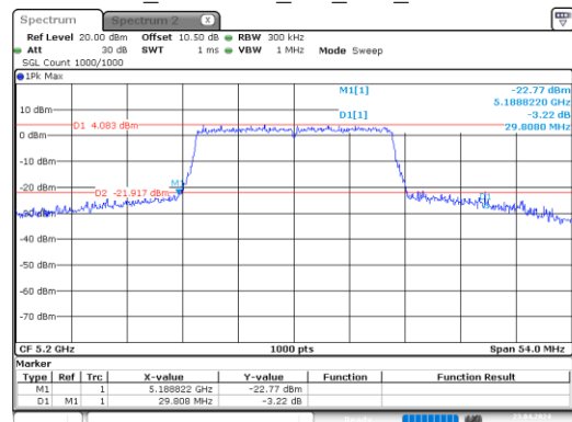
ax20_5200MHz_RU_Full_Chain 0
