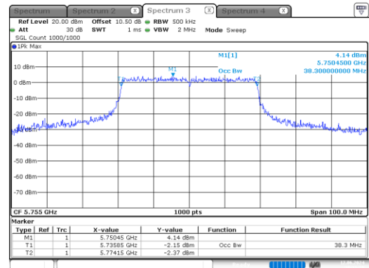
ax40_5755MHz_RU_Full_Chain 0
