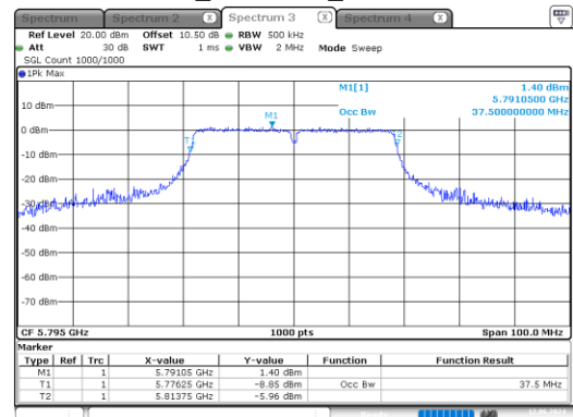
n40_5795MHz_Chain 0
