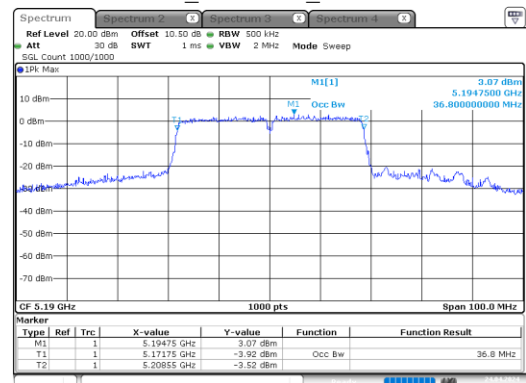
ac40_5190MHz_Chain 0
