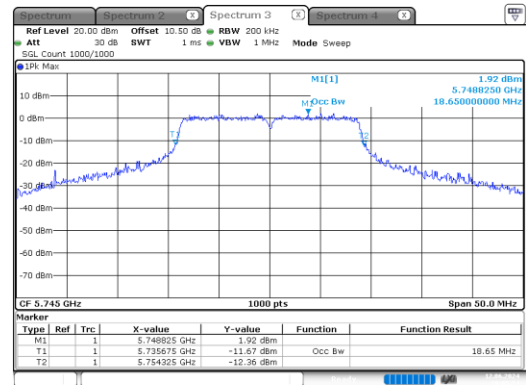
n20_5745MHz_Chain 0
