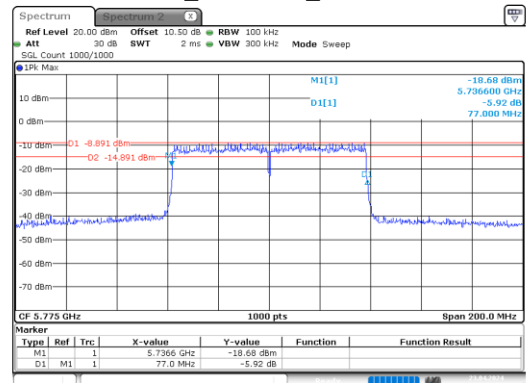
ac80_5775MHz_Chain 0
