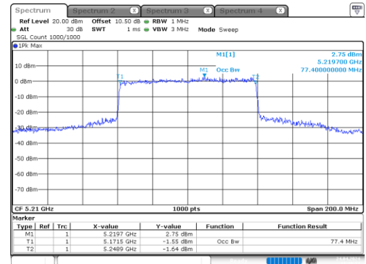
ax80_5210MHz_RU_Full_Chain 0
