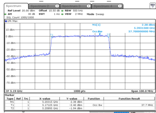
ax40_5190MHz_RU_Full_Chain 0
