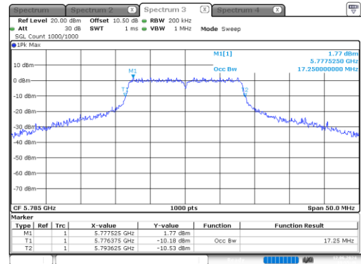
a_5785MHz_Chain 0
