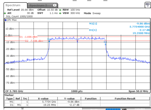
ax20_5785MHz_RU_Full_Chain 0
