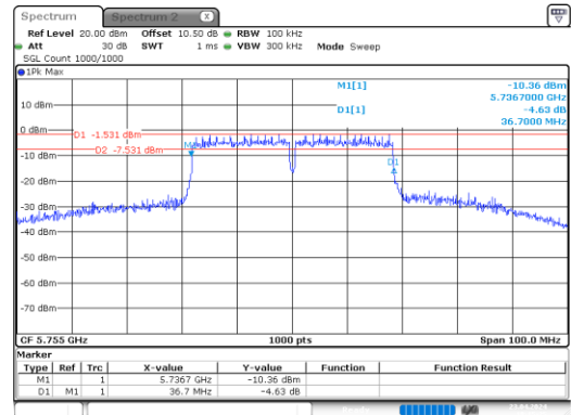
ac40_5755MHz_Chain 0
