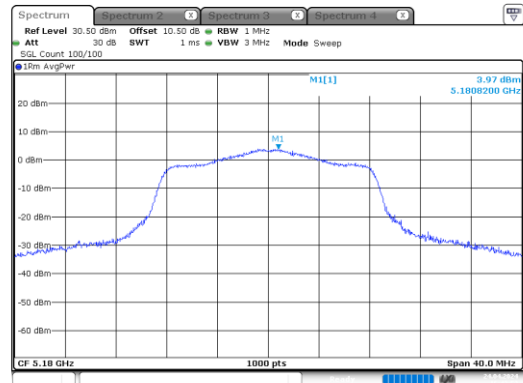
a_5180MHz_Chain 1
