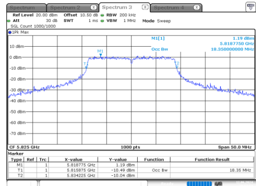
n20_5825MHz_Chain 0
