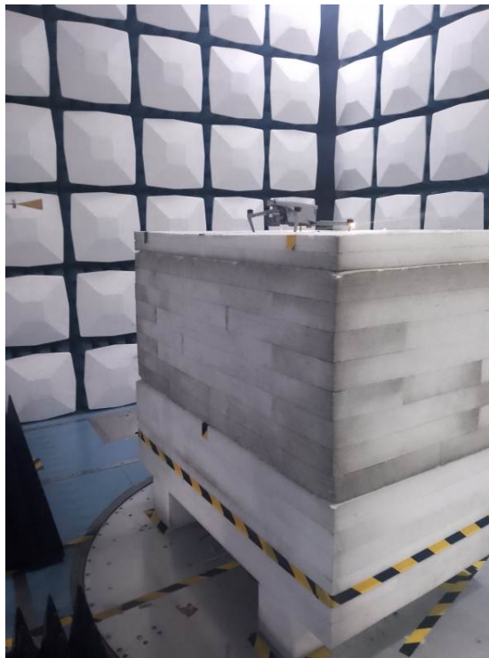
Radiated Emission 40-60GHz View
