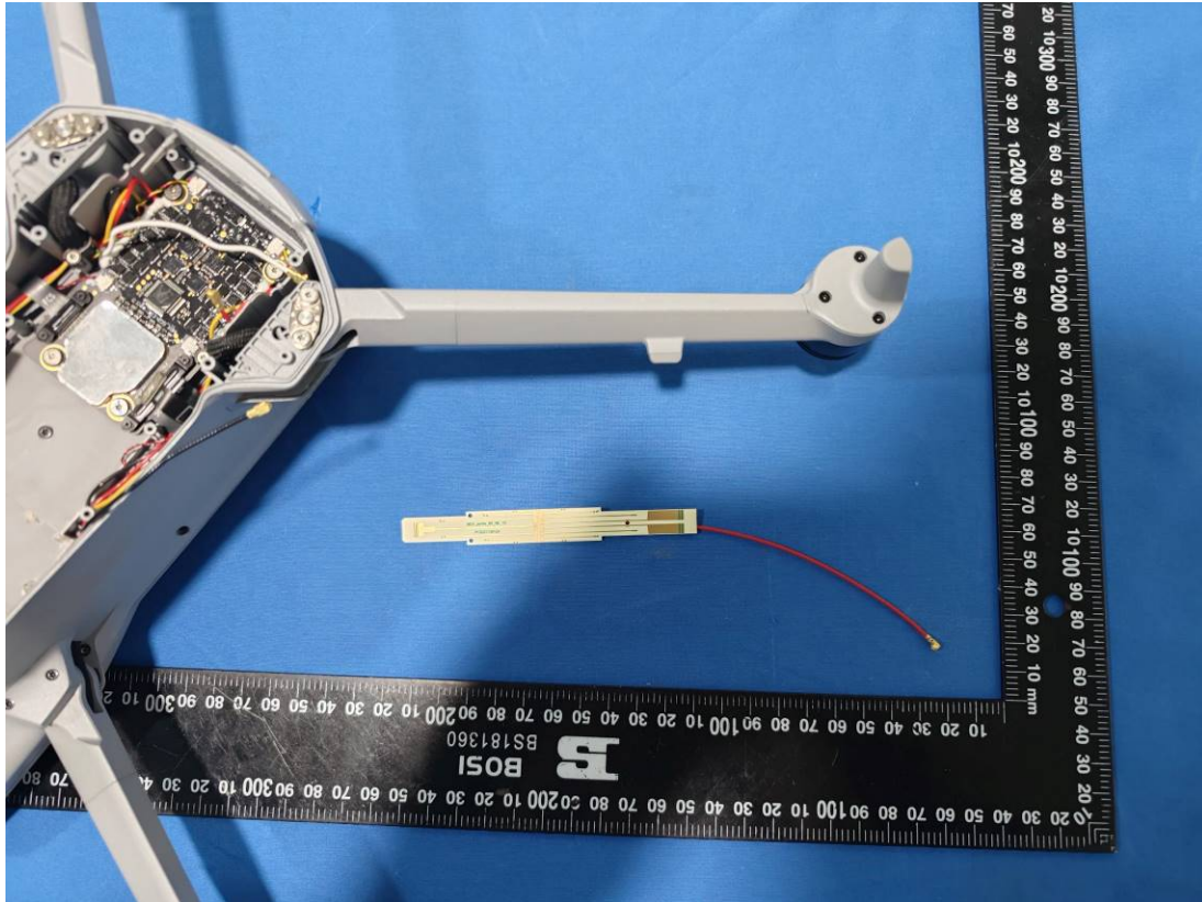
SRD Antenna 3(Back Right)
