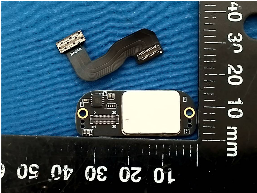
Rear Radar
