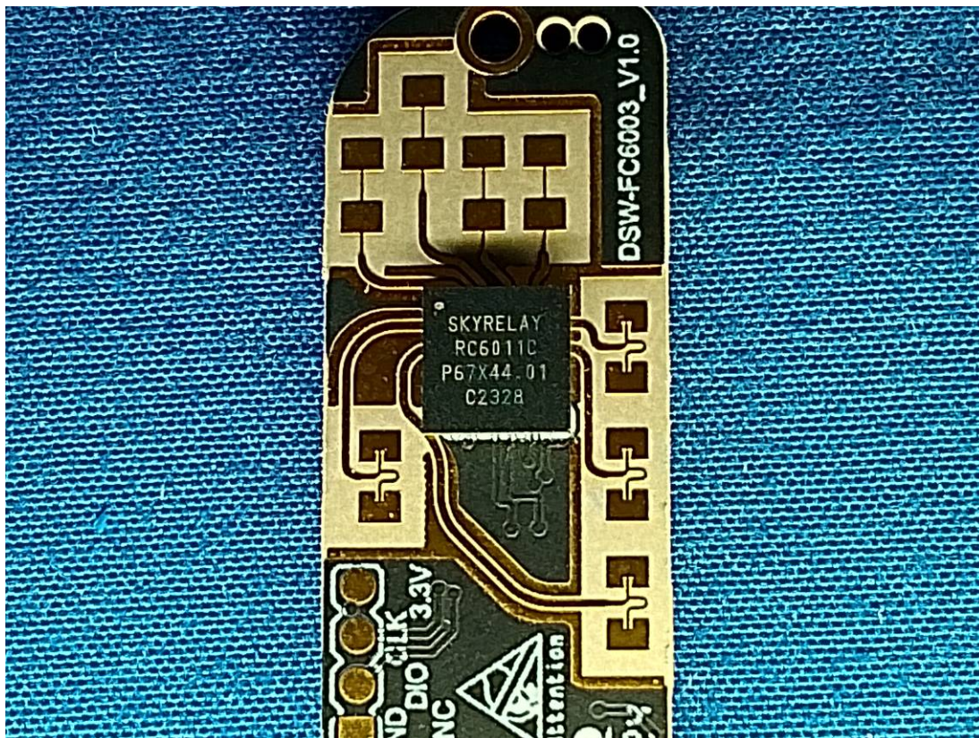
Radar Chip+ANT
