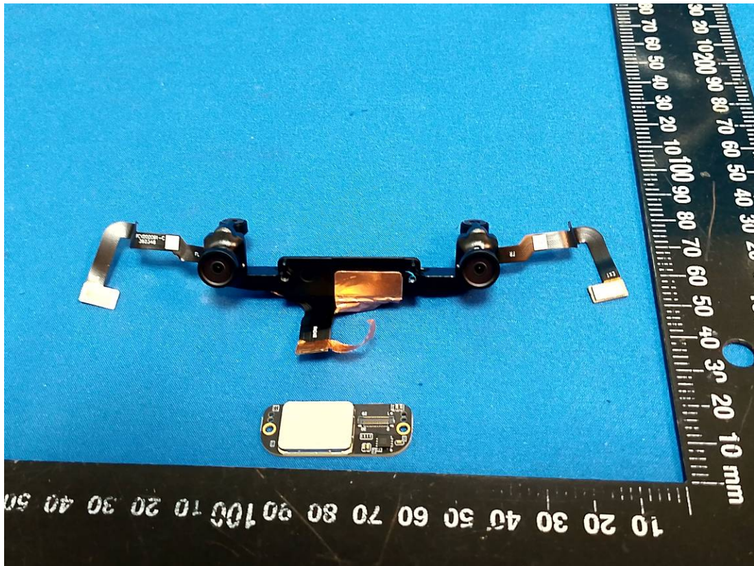
Front Radar
