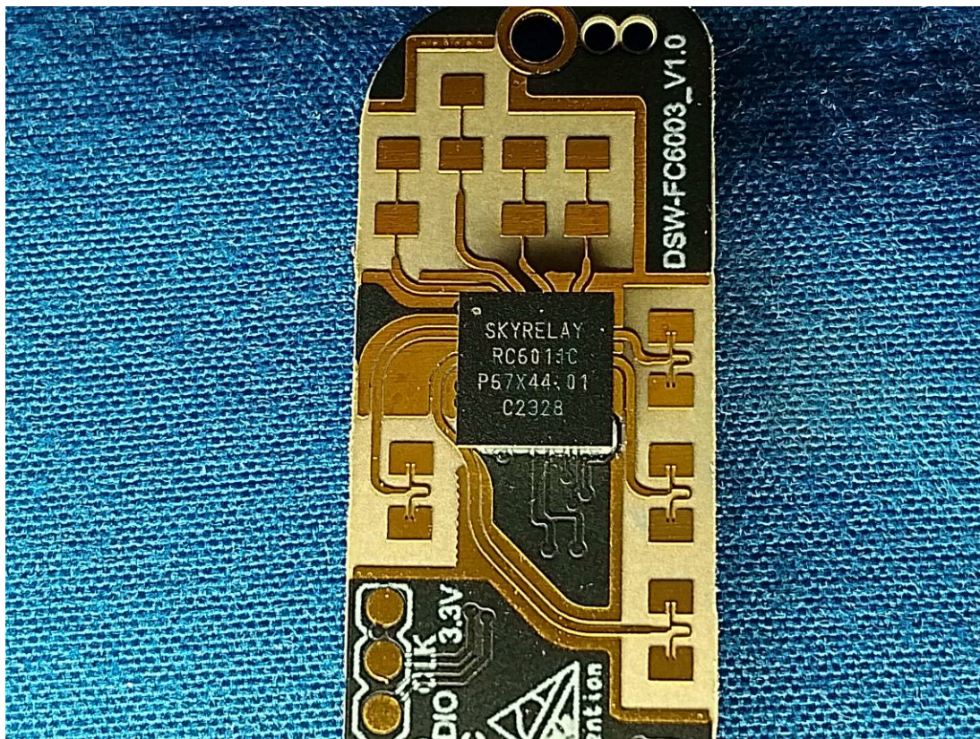
Front Radar Chip+ANT
