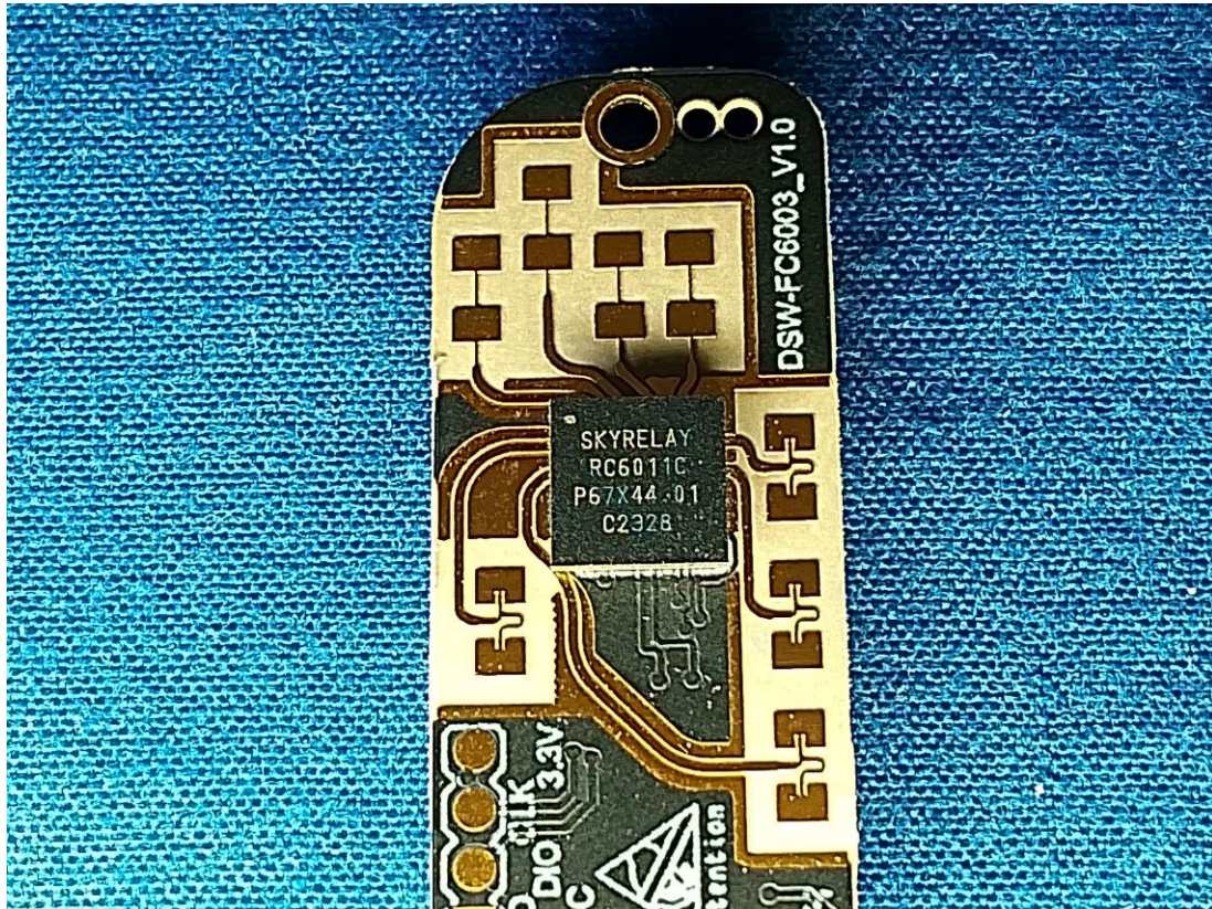
Bottom Radar Chip+ANT
