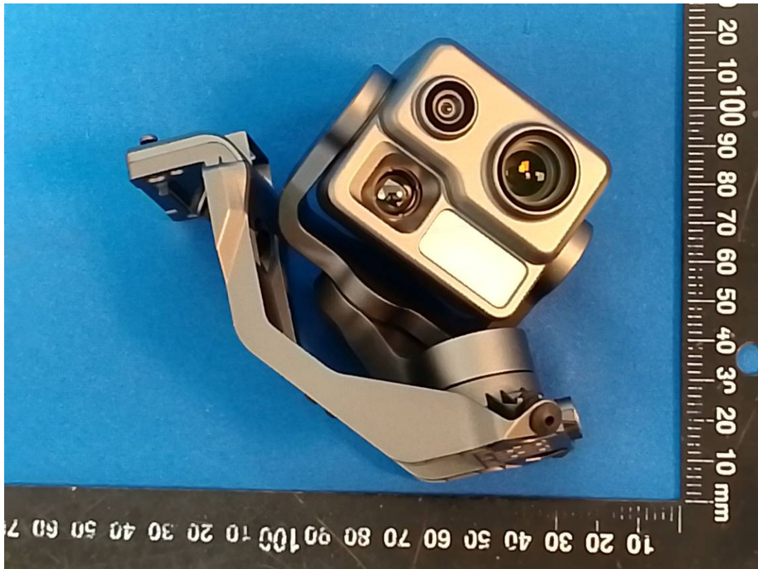
Gimbal camera 2#(Fusion 4NZ) For PMN: EVO Max 4NZ V2
