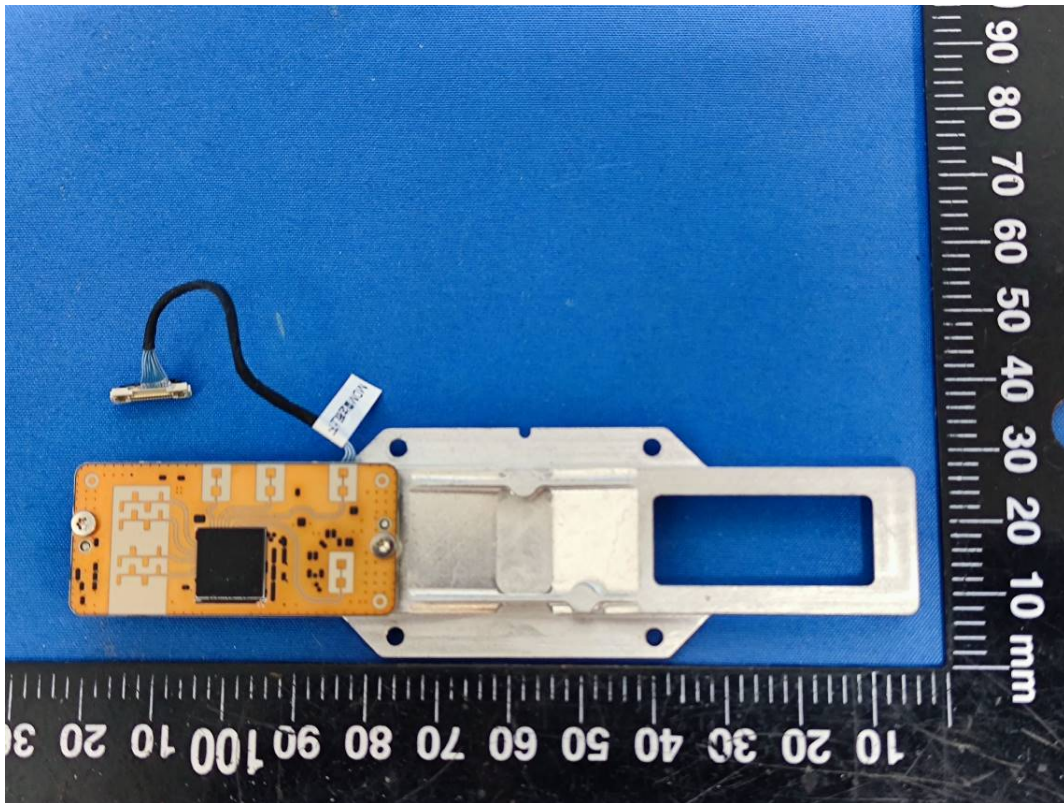
Rear Radar(Low Band)
