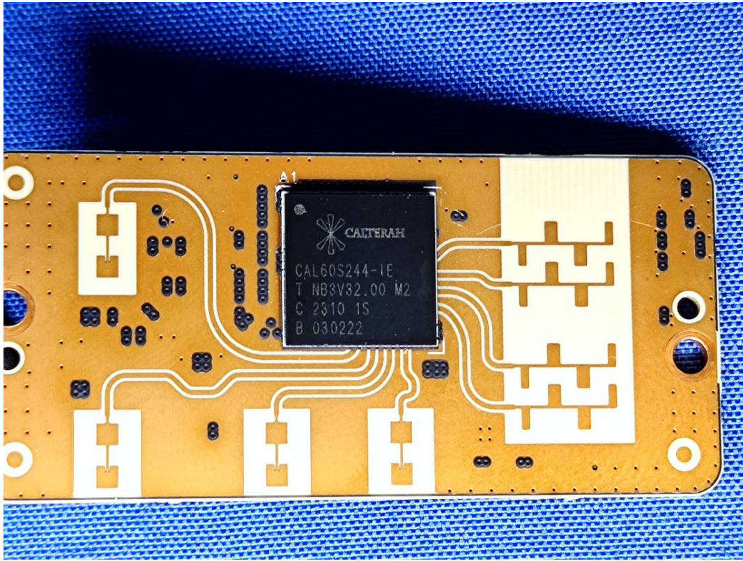
Chip+Antenna
