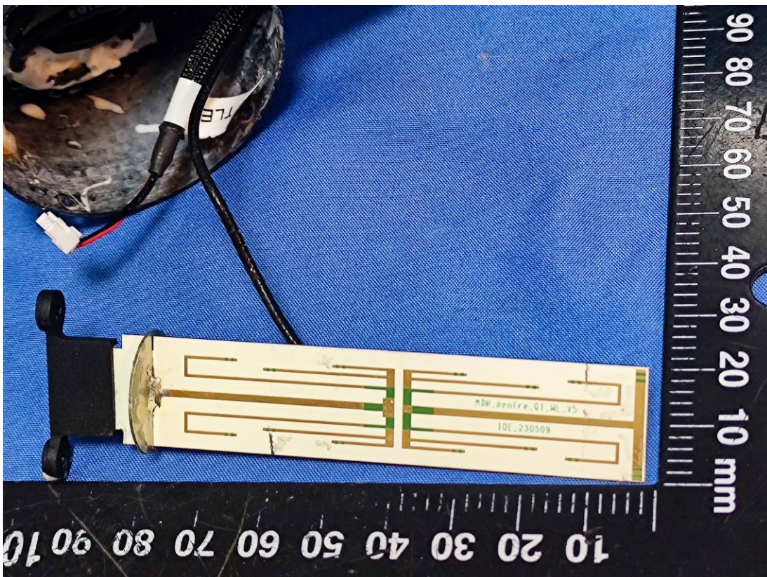
SRD Antenna 1
