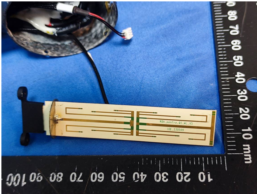
SRD Antenna 0
