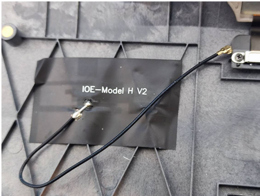
ADS-B Antenna
