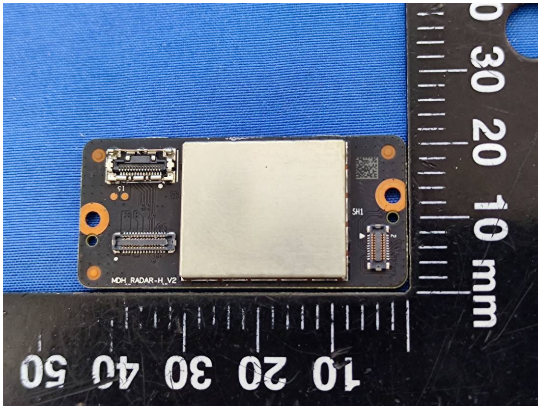
Bottom Radar Module(High Band)
