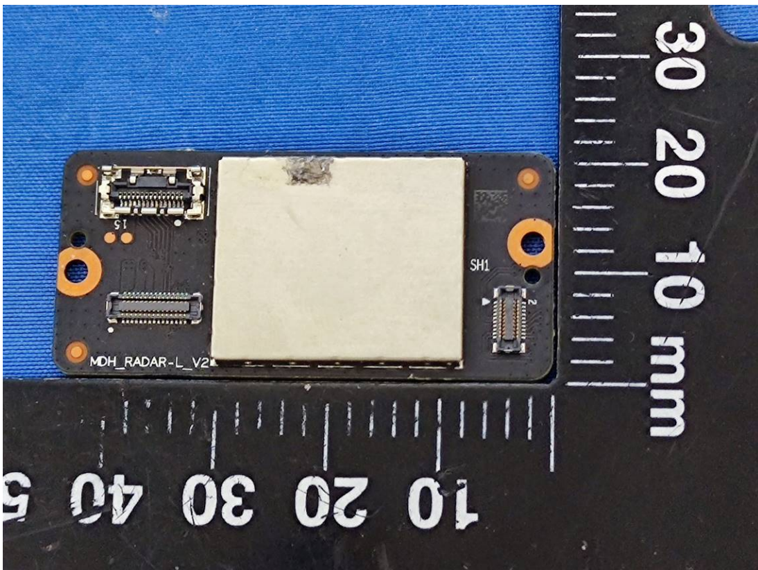
Back Radar(Low Band)
