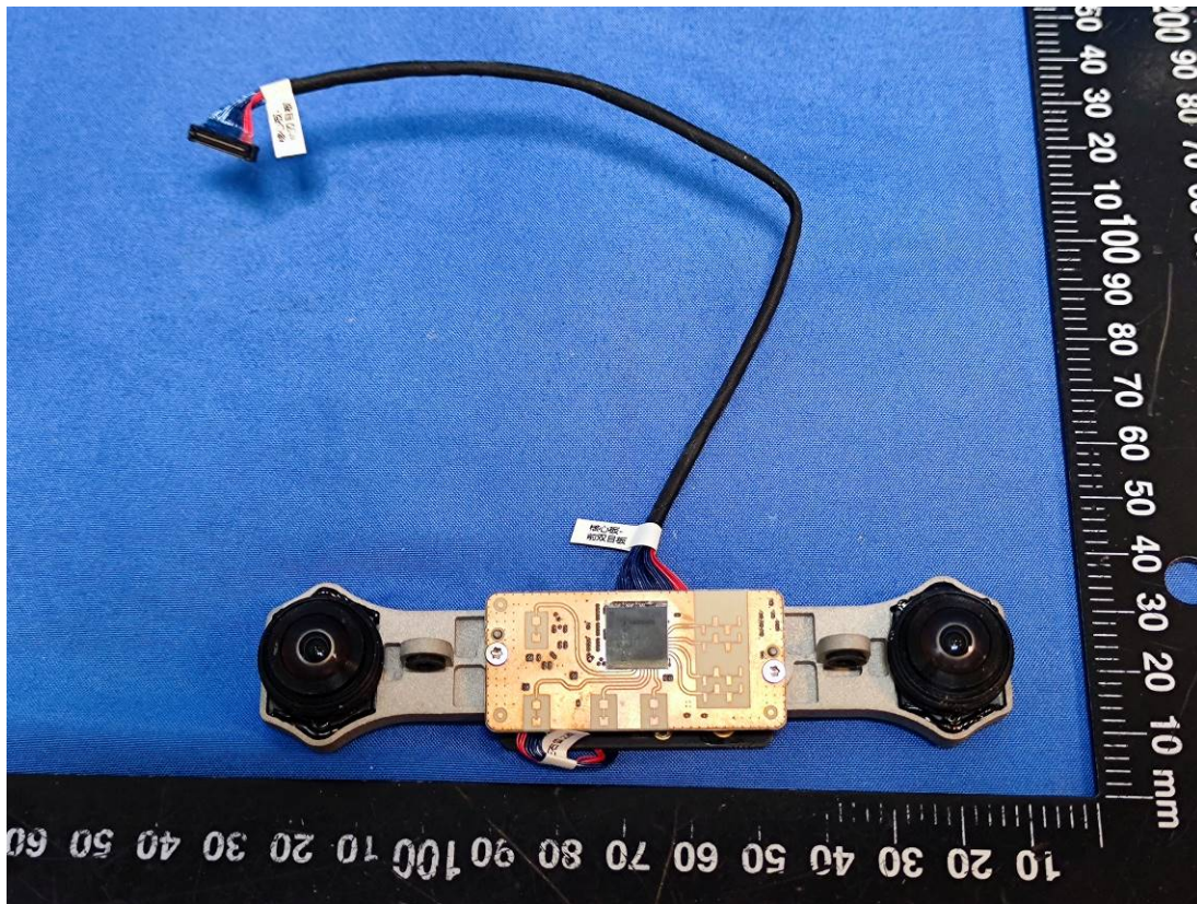
Front Radar(High Band)
