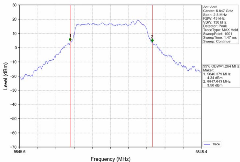
16QAM_HCH_5847MHz_Ant1_NTNV
