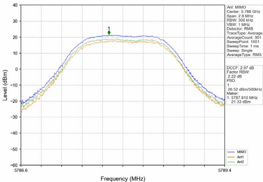
QPSK_MCH_5788MHz_MIMO_NTNV
