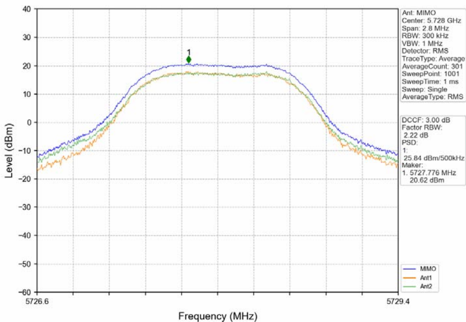
16QAM_LCH_5728MHz_MIMO_NTNV
