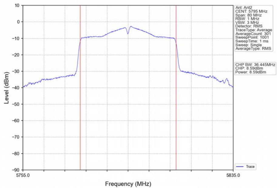
802.11ac(VHT40)_HCH_5795MHz_Ant2_NTNV
