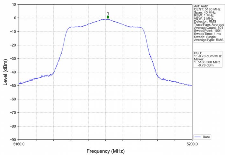
802.11ac(VHT20)_LCH_5180MHz_Ant2_NTNV
