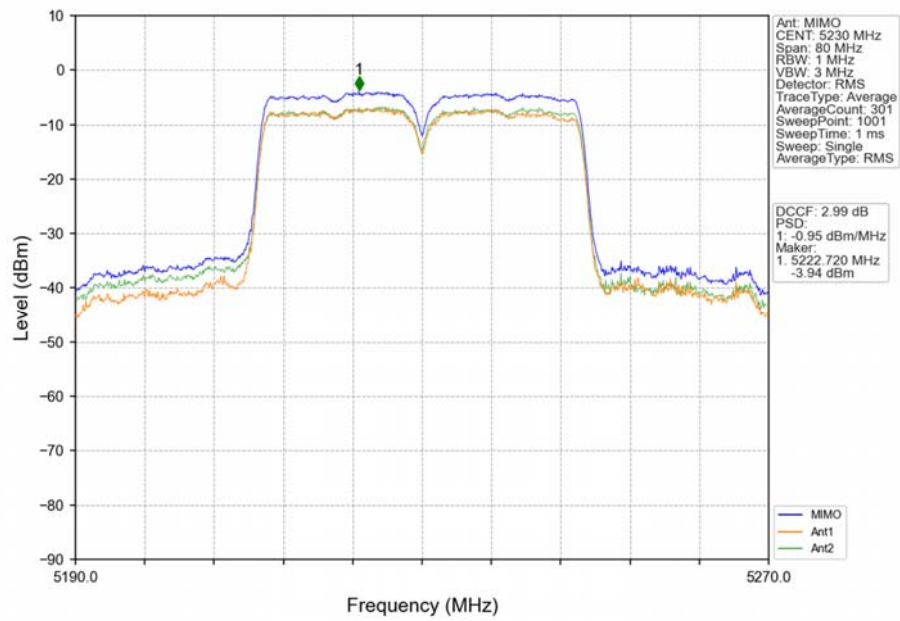
802.11n(HT40)_HCH_5230MHz_MIMO_NTNV
