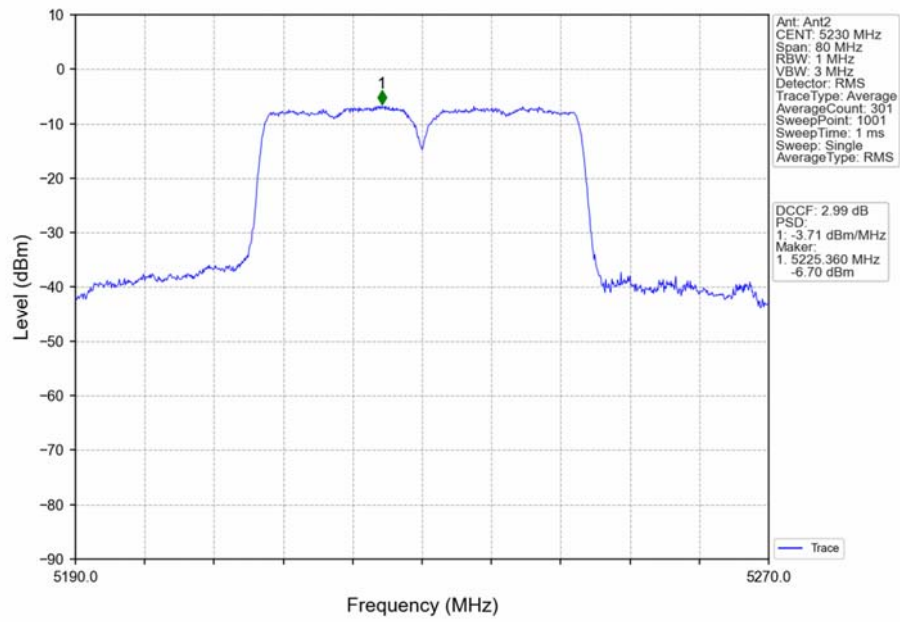
802.11n(HT40)_HCH_5230MHz_MIMO_NTNV
