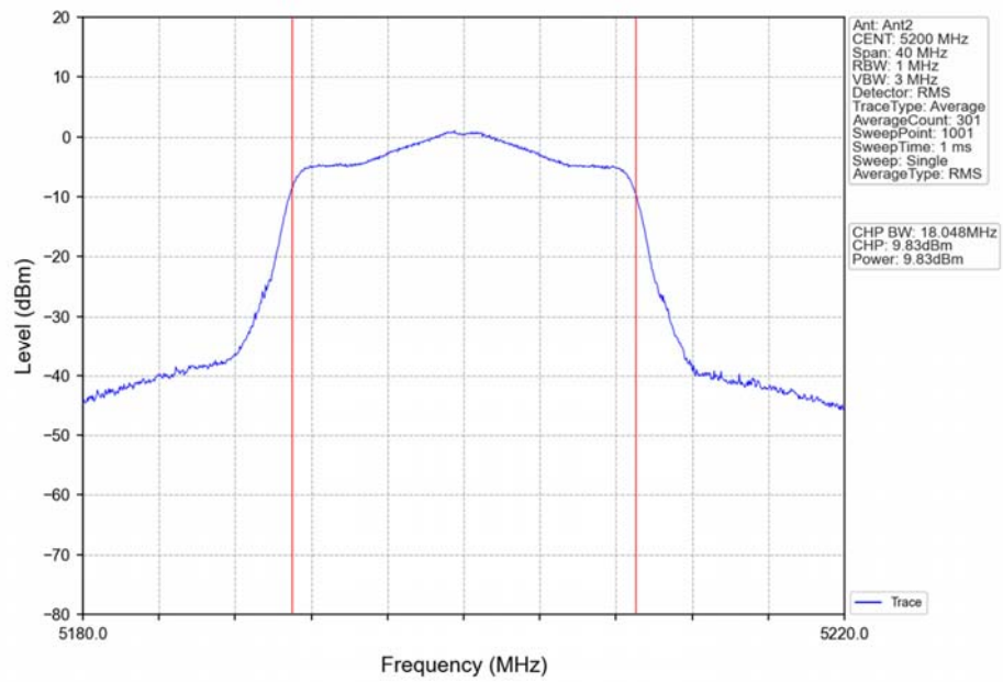
802.11ac(VHT20)_MCH_5200MHz_Ant2_NTNV
