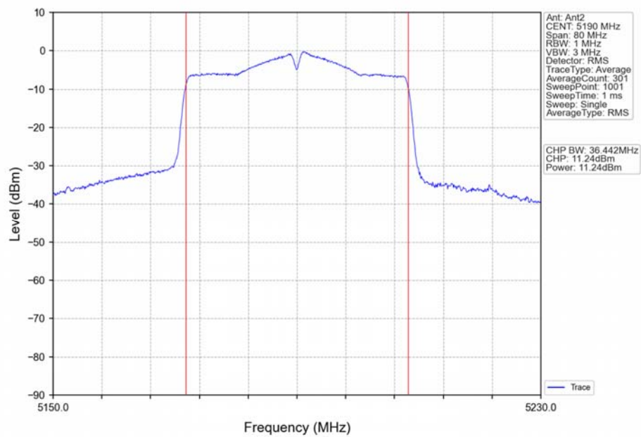
802.11ac(VHT40)_LCH_5190MHz_Ant2_NTNV
