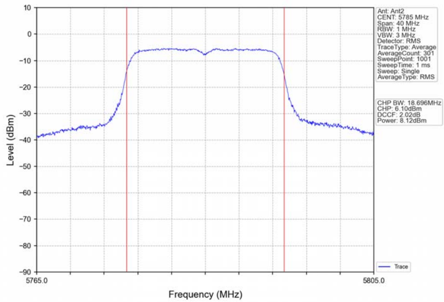
802.11n(HT20)_MCH_5785MHz_Ant2_NTNV
