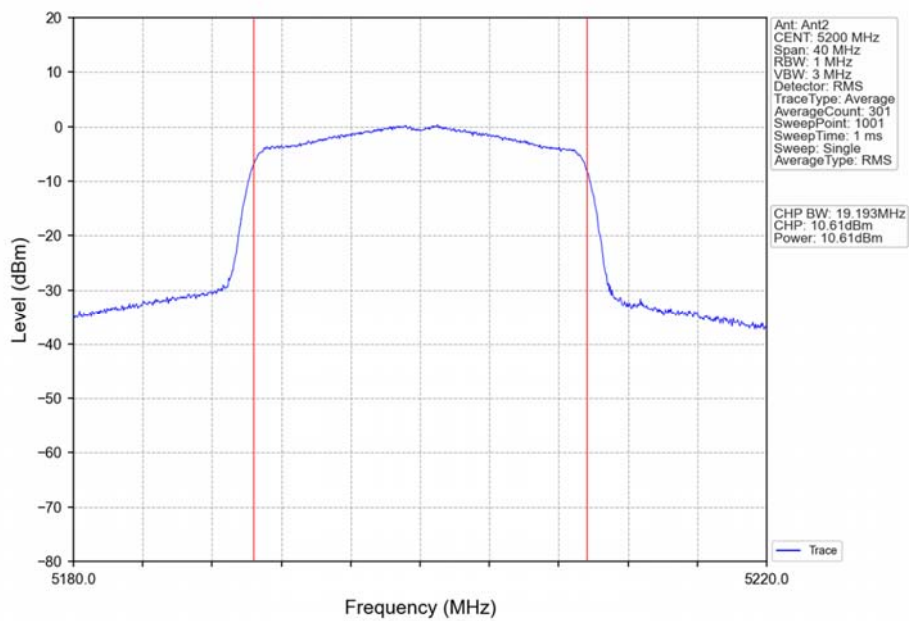
802.11ax(HEW20)_MCH_5200MHz_RU242_Left_Ant2_NTNV
