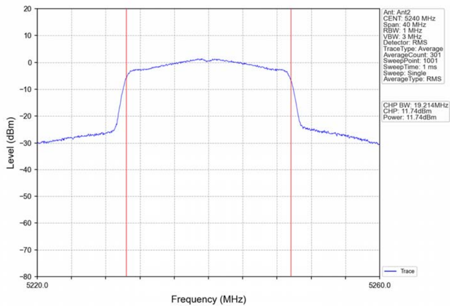
802.11ax(HEW20)_HCH_5240MHz_RU242_Left_Ant2_NTNV
