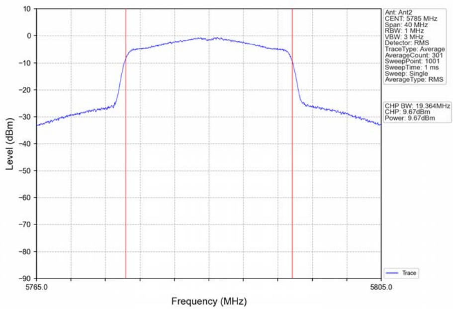
802.11ax(HEW20)_MCH_5785MHz_RU242_Left_Ant2_NTNV
