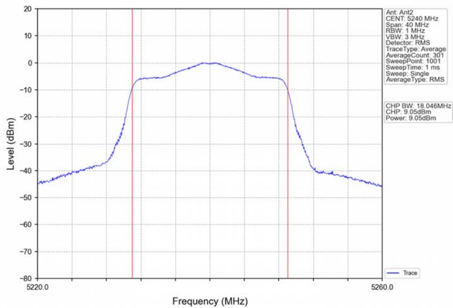
802.11ac(VHT20)_HCH_5240MHz_Ant2_NTNV
