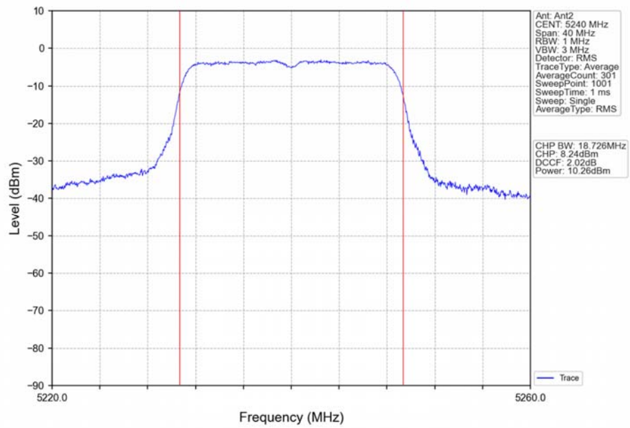
802.11n(HT20)_HCH_5240MHz_Ant2_NTNV
