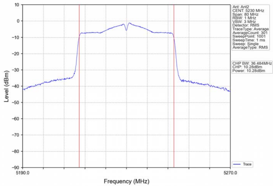
802.11ac(VHT40)_HCH_5230MHz_Ant2_NTNV
