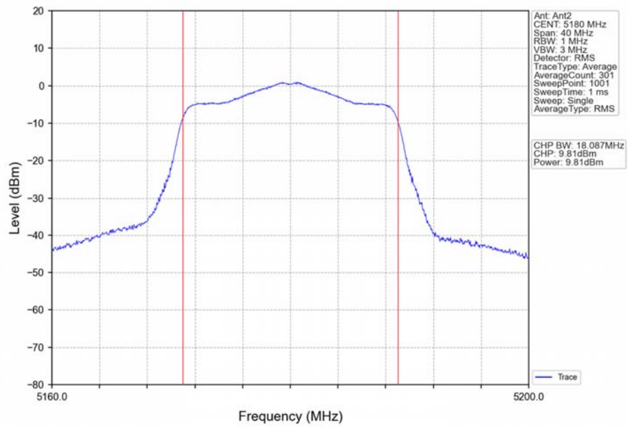
802.11ac(VHT20)_LCH_5180MHz_Ant2_NTNV
