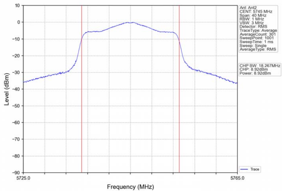
802.11ac(VHT20)_LCH_5745MHz_Ant2_NTNV
