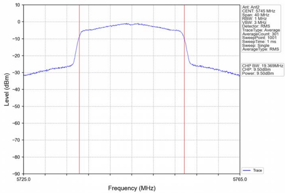
802.11ax(HEW20)_LCH_5745MHz_RU242_Left_Ant2_NTNV
