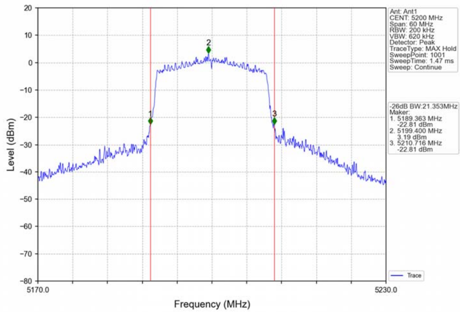
802.11ax(HEW20)_MCH_5200MHz_RU242_Left_Ant1_NTNV
