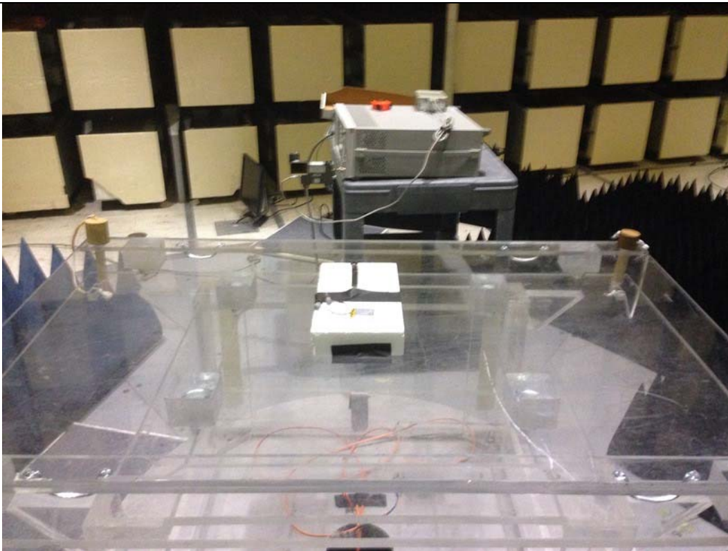
Radiated Spurious, 18-26 GHz, Back
