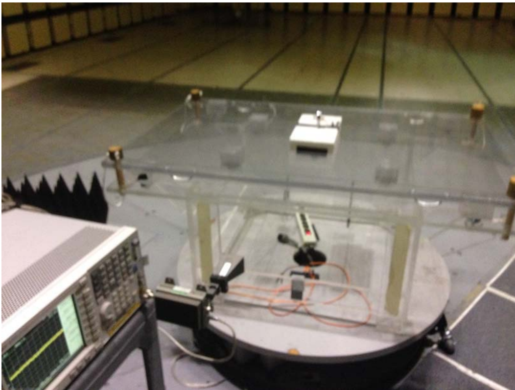
Radiated Spurious, 18-26 GHz, Front
