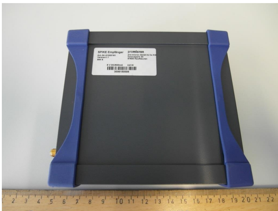
Photo 2: Receiver
