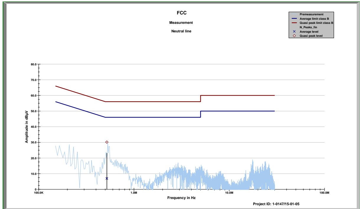
Plot 2: 150 kHz to 30 MHz, neutral line
