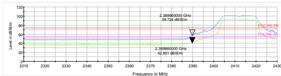
802.11g-Channel 1 Peak +Average
