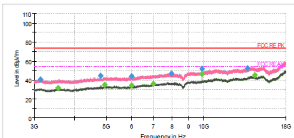
Radiated Emission from 3GHz to 18GHz
