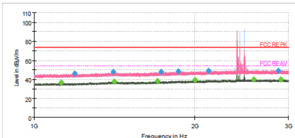
Radiated Emission from 1GHz to 3GHz
