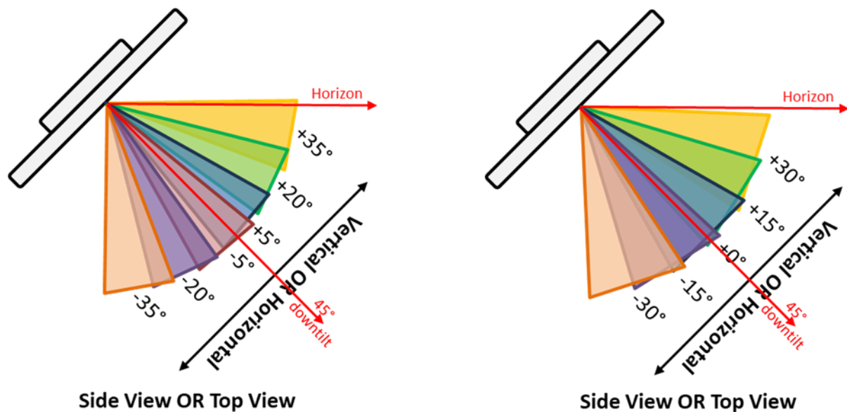
Figure 3: AP750NRe AP Radiation Pattern
