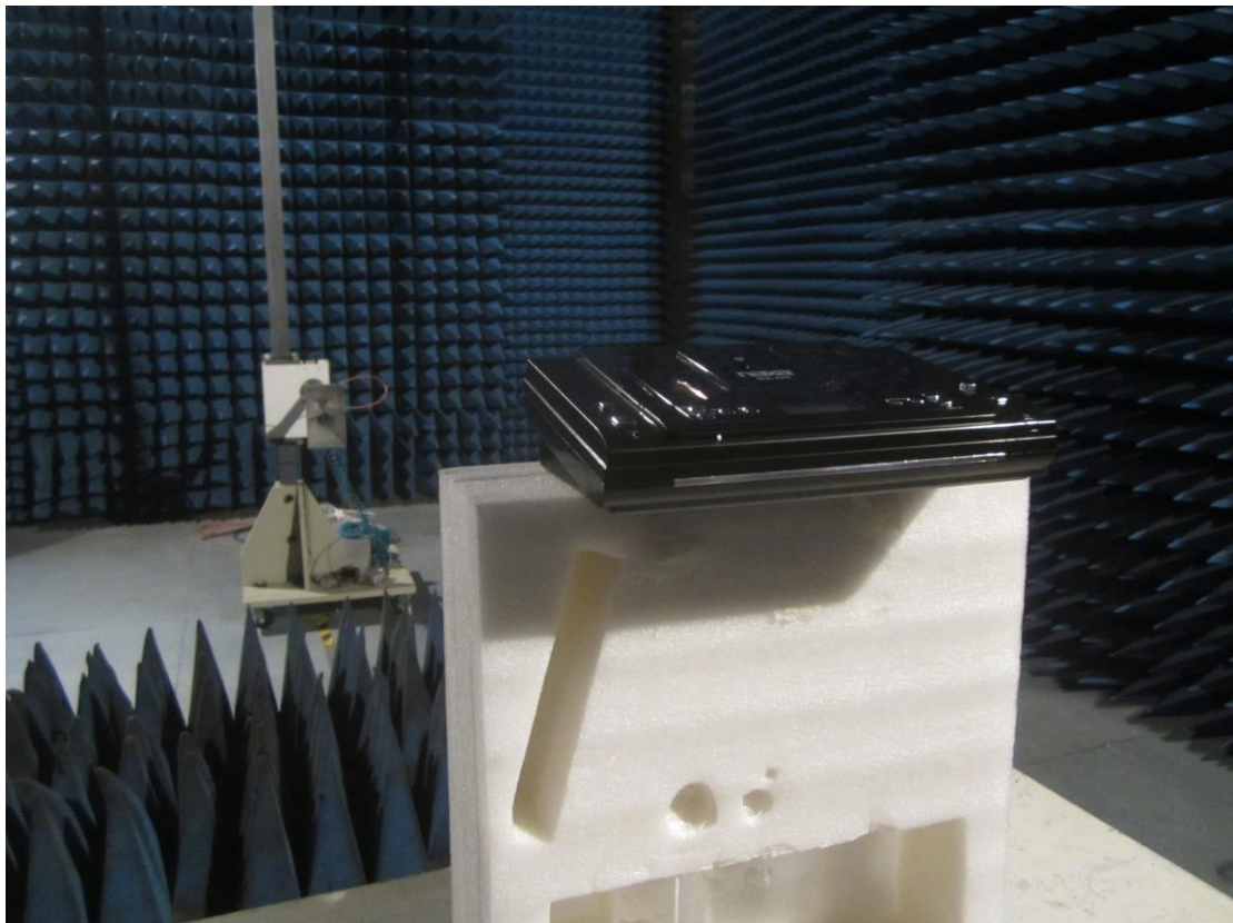
Setup for Radiated emission:
