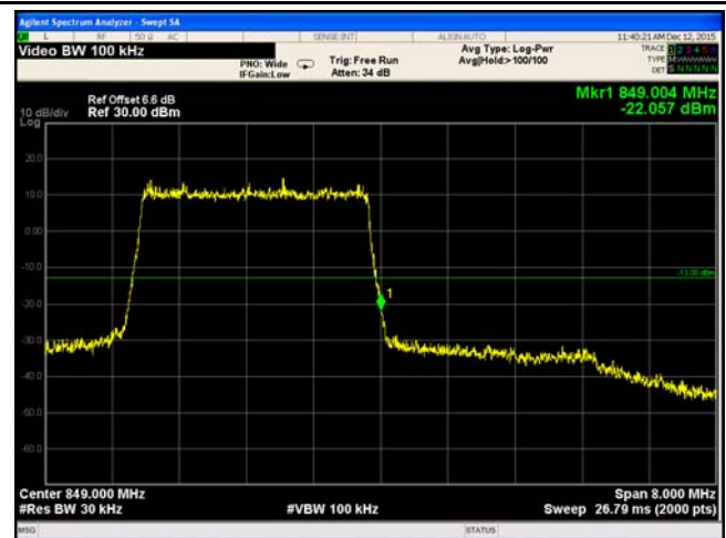
LTE Band 5 - High Channel 16QAM-3
