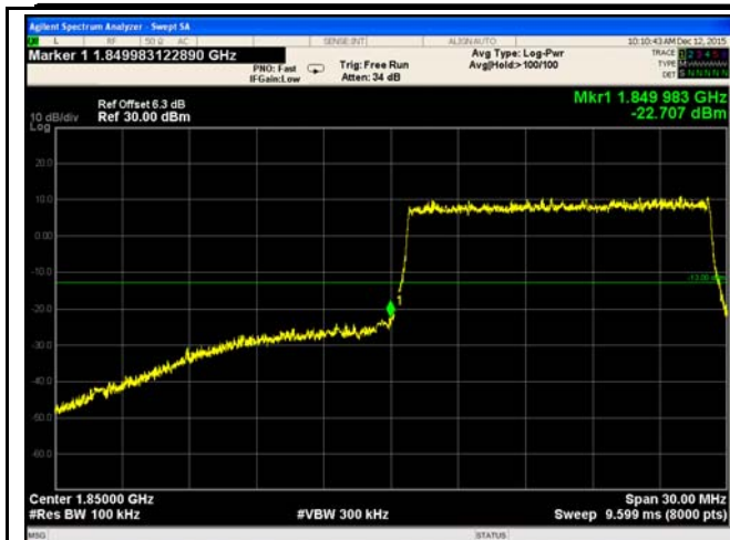
LTE Band 2 - Low Channel QPSK-15
