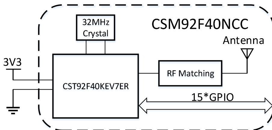
Figure 1.2 CSM92F40NCC module Function Block Diagram (chip antenna)
