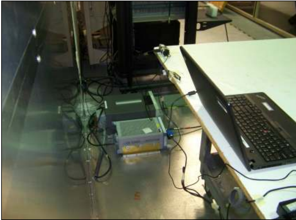
Figure 9: Conducted Emissions – Attached Eval Board
