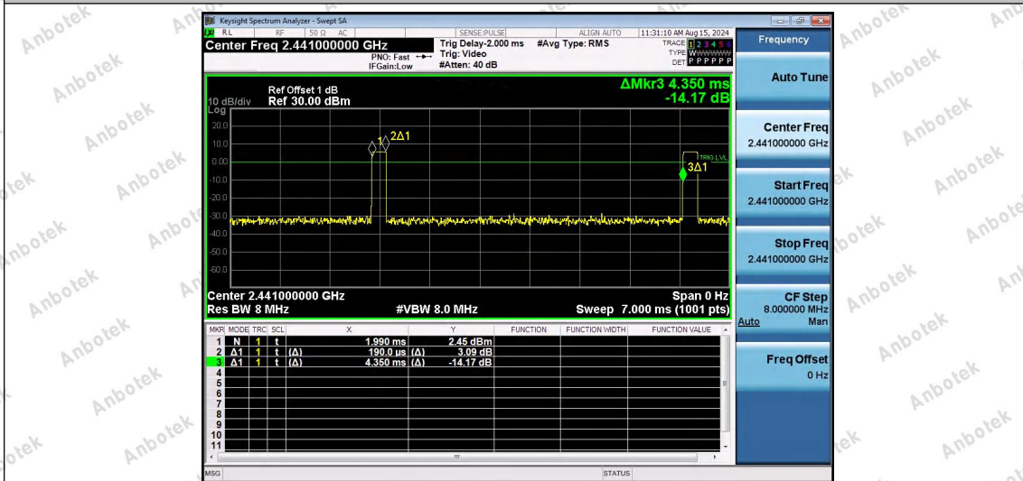
NTNV-2.4G-Ant1-2441
