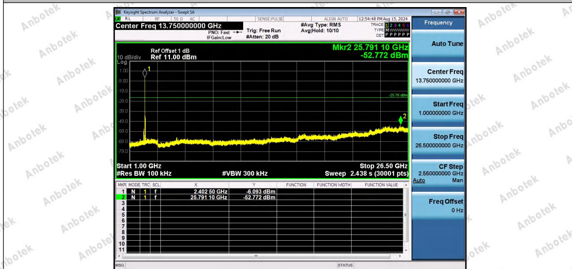
2.4G-Ant1-2403-1000~26500-PASS
