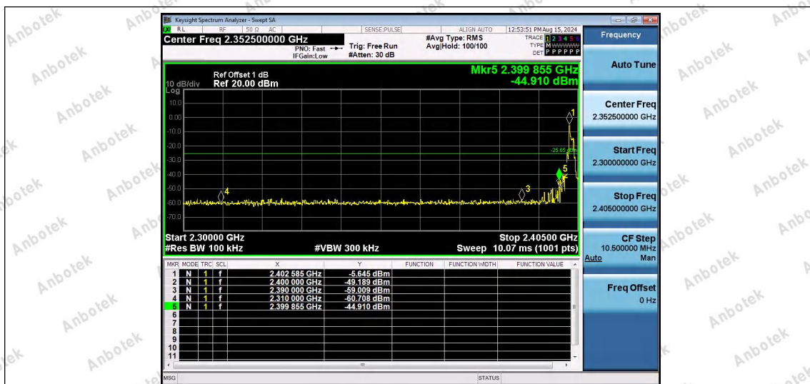
2.4G-Ant1-2403-PASS
