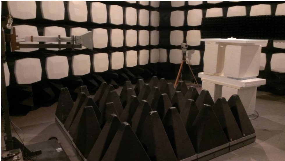
Radiated measurements 1-10 GHz
