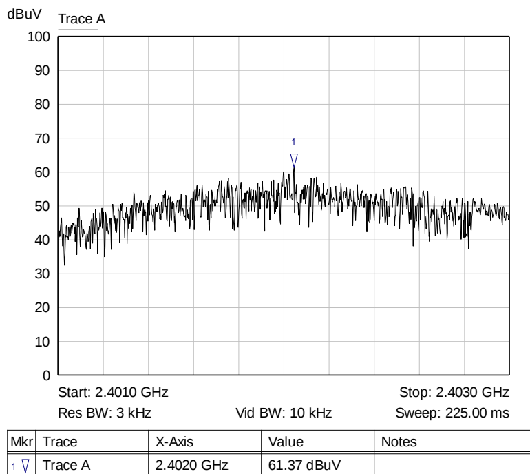
Graph 9: Lowest Channel 3 kHz PSD Plot
