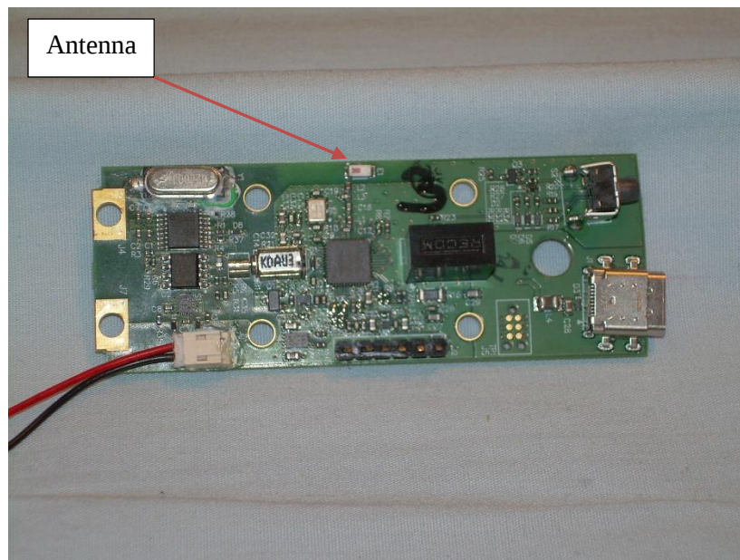
Photograph 14: Top View of the PCB
