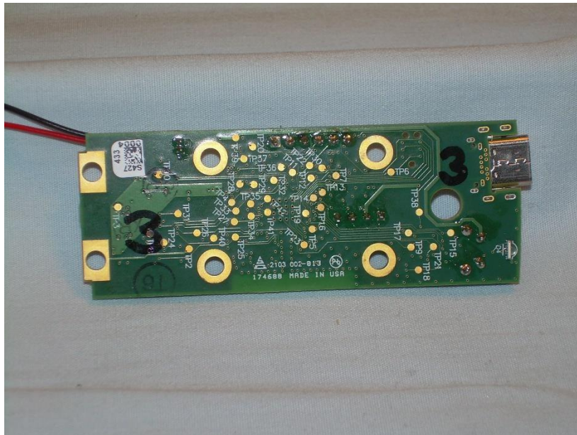
Photograph 15: Bottom View of the PCB
