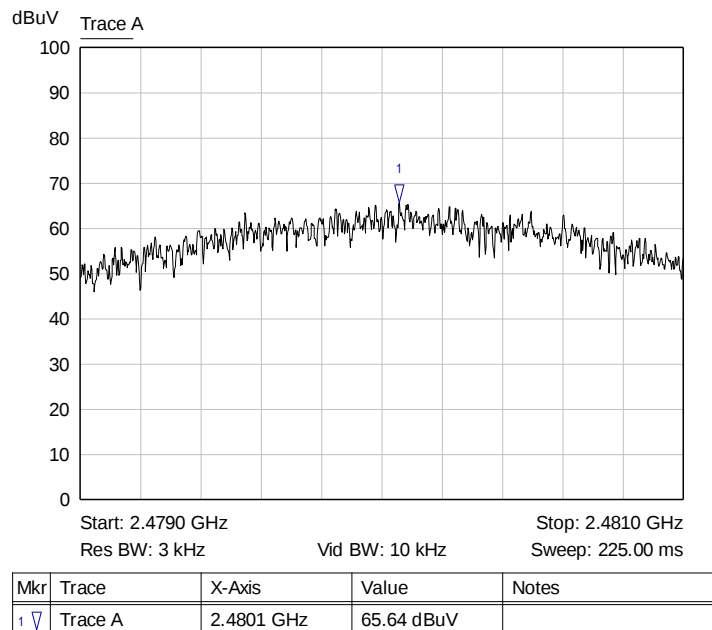
Graph 11: Highest Channel Output 3 kHz PSD Plot
