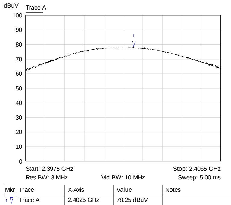
Graph 4: Lowest Channel Output Power Plot
