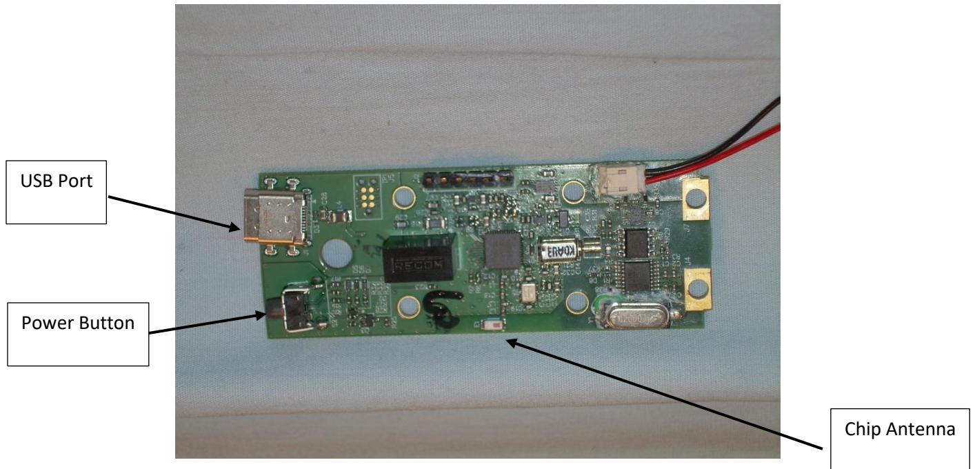
Photograph 1 – Top View of the PCB with Shield
