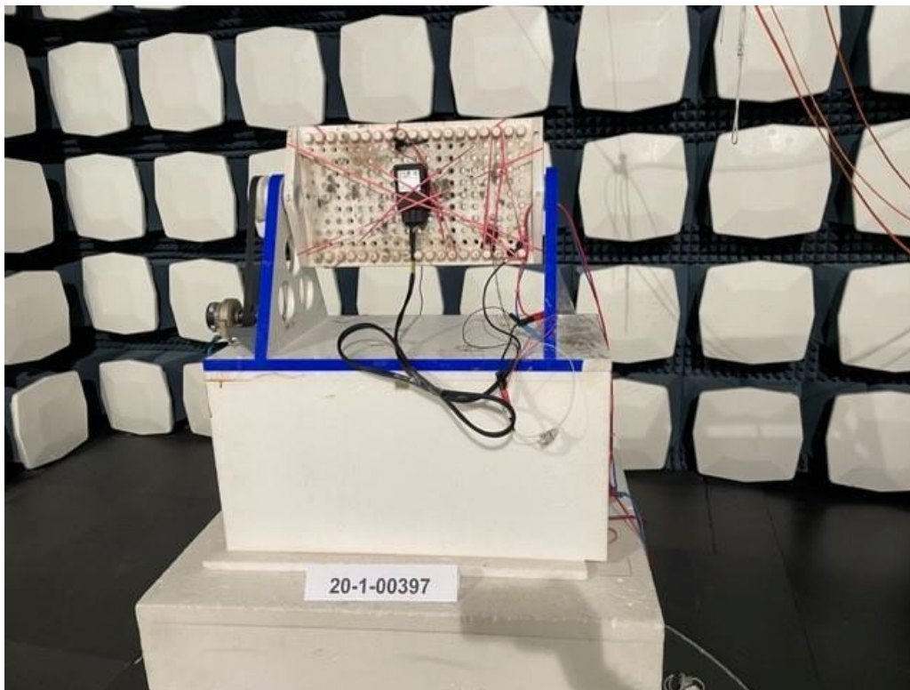
Fig. Mea.: 3 : Measurements in the fully anechoic chamber 1
