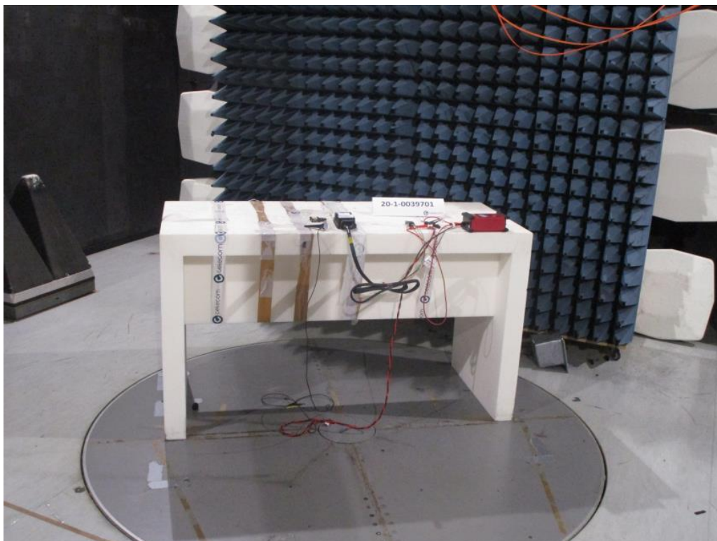
Fig. Mea.: 2 : Measurements in the semi anechoic chamber
