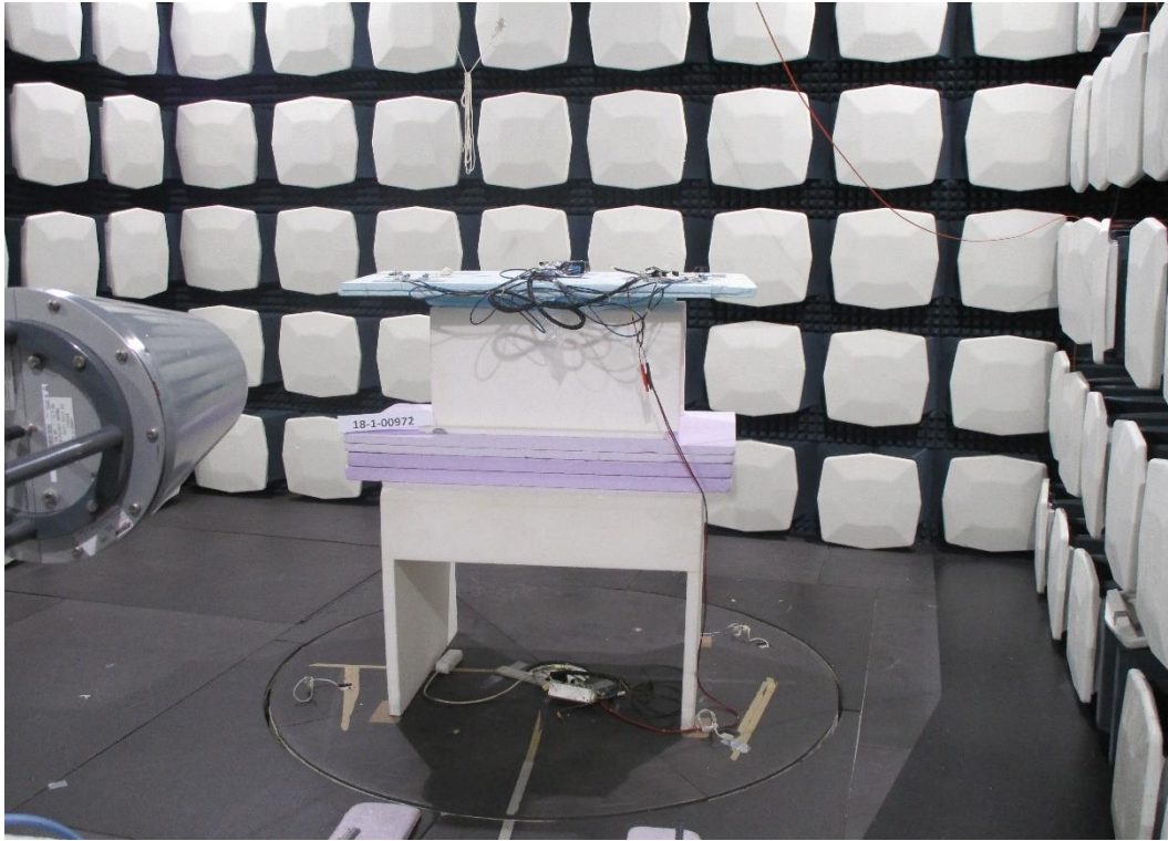
EUT setup (EUT Position Laying)
