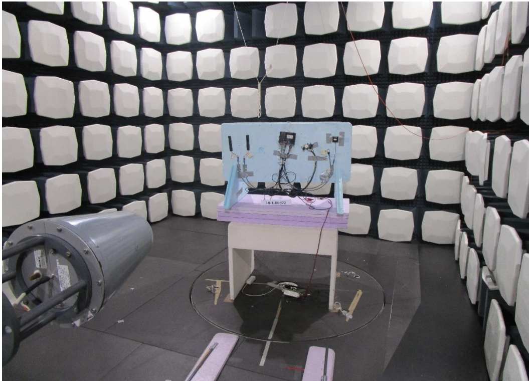
EUT setup overall view (EUT Position Standing)
