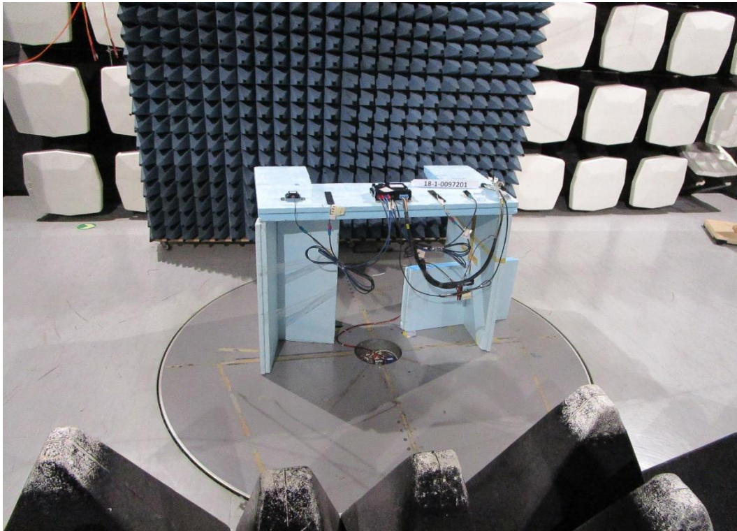
Closed-up view_EUT setup Laying Position
