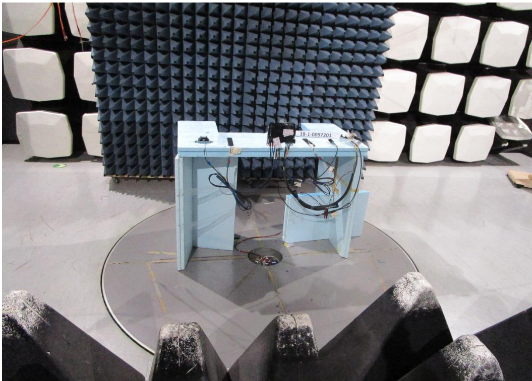
Closed-up view_EUT setup Standing Position
