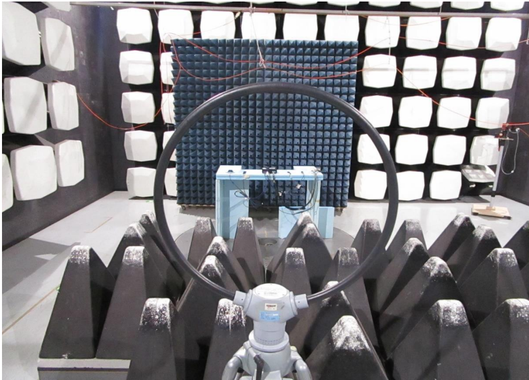
Overall view_EUT setup Laying Position
