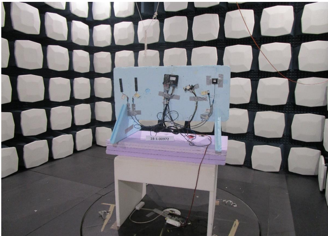
EUT setup (EUT Position Standing)
