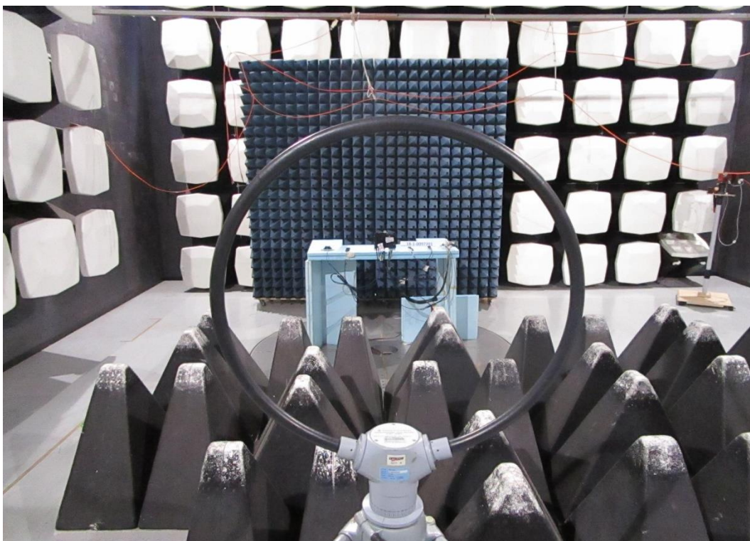
Overall view_EUT setup Standing Position
