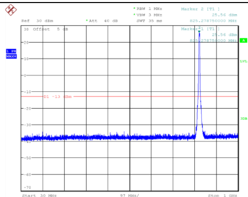
Channel 4133: 30MHz~1GHz
