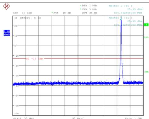
Channel 4175: 30MHz~1GHz
