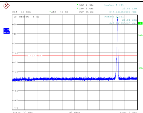
Channel 4232: 30MHz~1GHz
