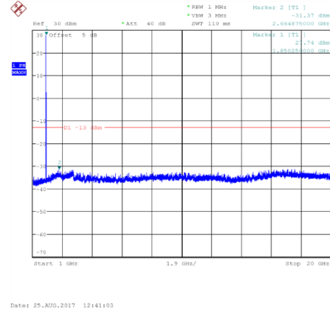
Channel 661: 1GHz~20GHz
