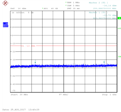
Channel 661: 30MHz~1GHz
