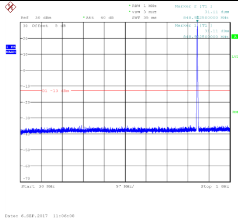
Channel 251: 30MHz~1GHz
