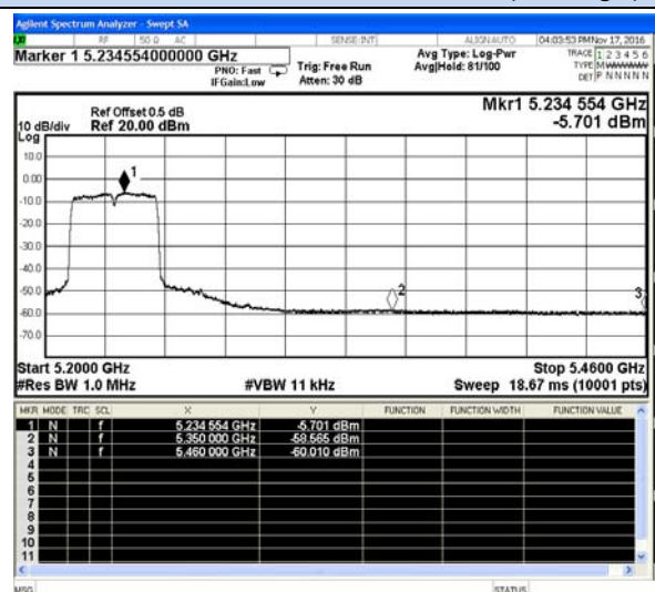
802.11n-HT40-High channel(Average)
