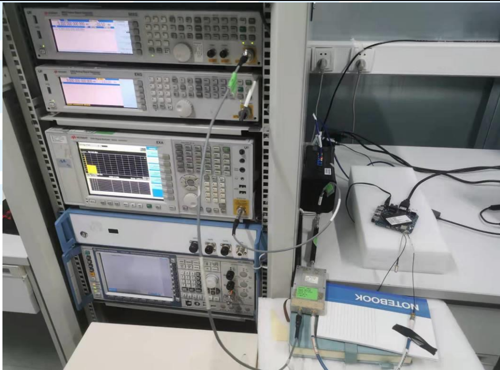
DFS Test Setup
