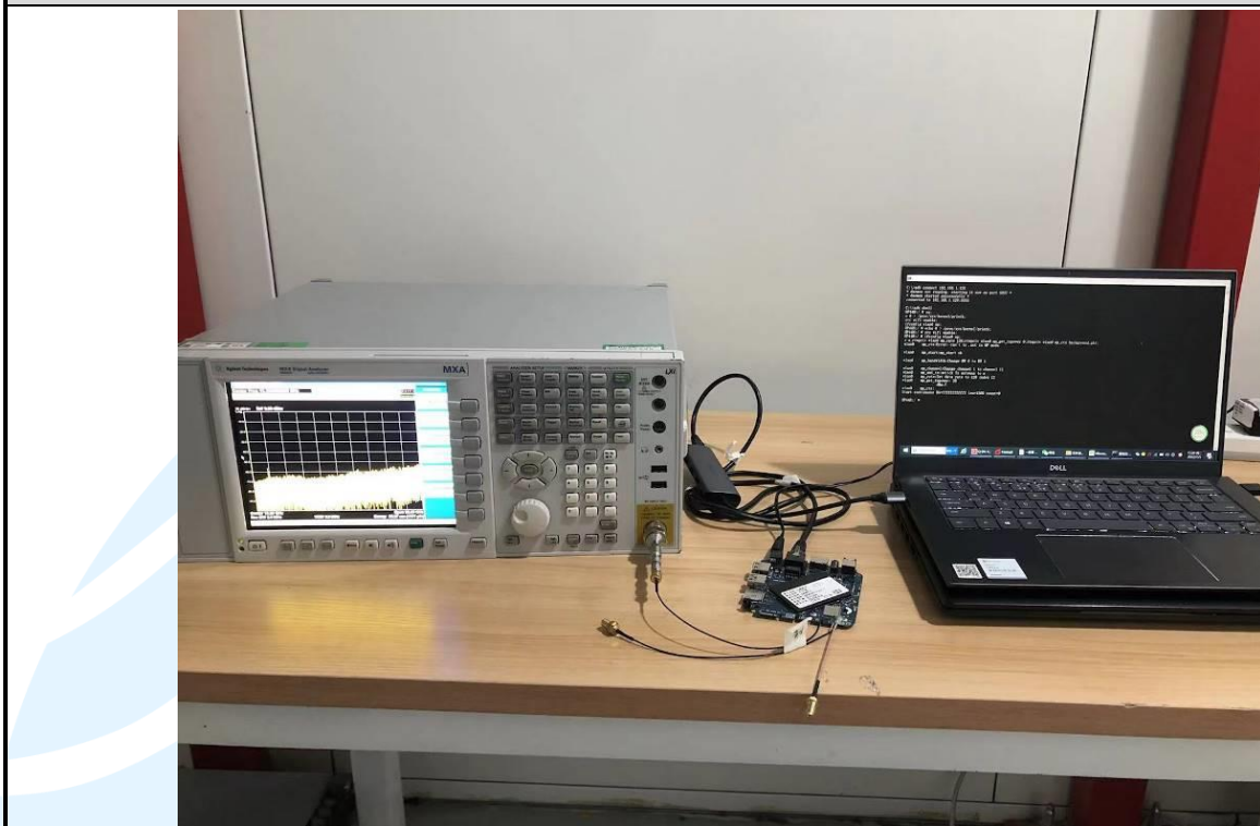
RF Test Setup
