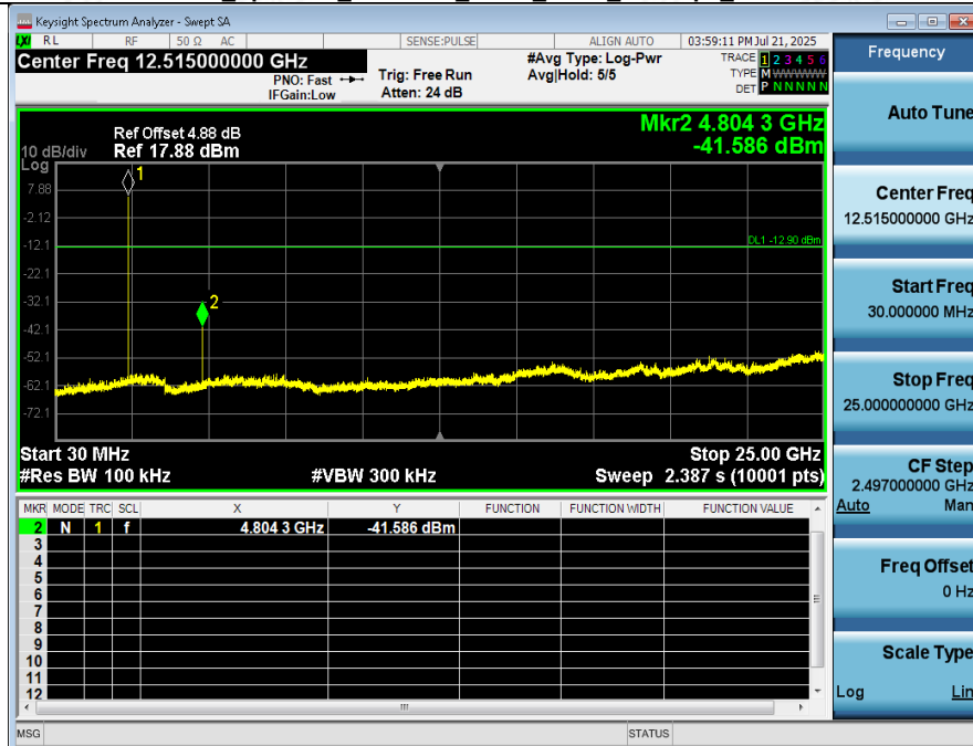
2_Spurious_Emission_NVNT_ANT1_500 kbps_2402
