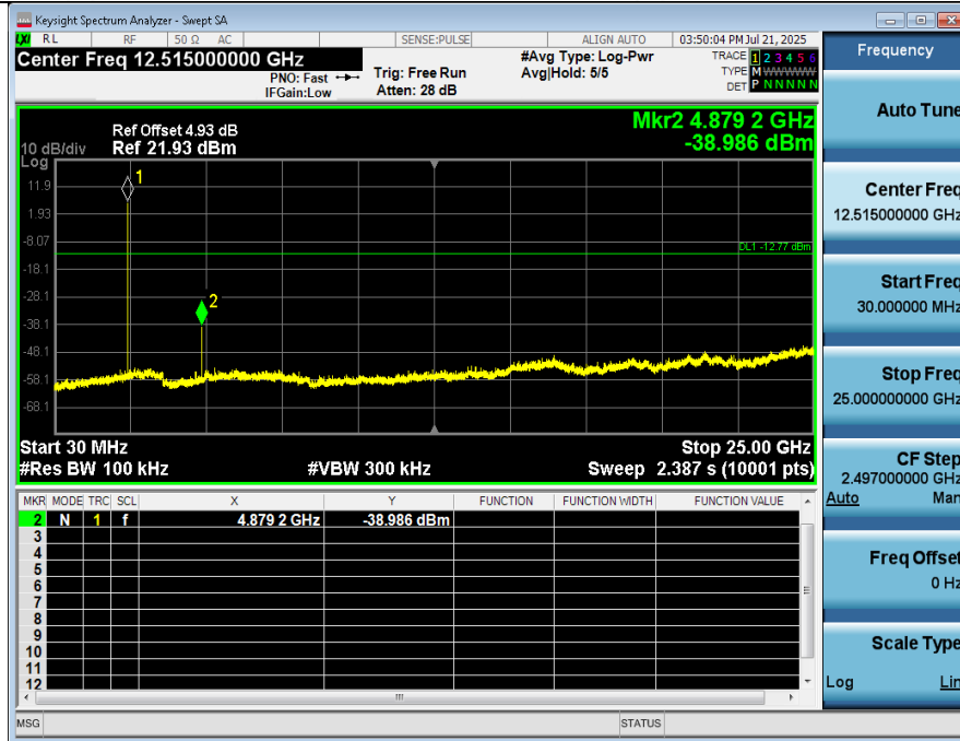
2_Spurious_Emission_NVNT_ANT1_500 kbps_2440
