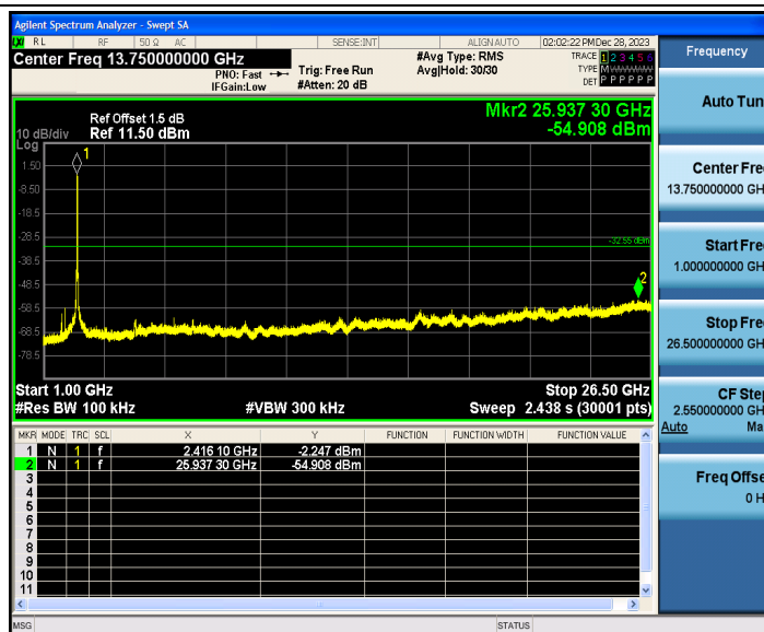
802.11n(HT40)_Ant1_2437_0~Reference
