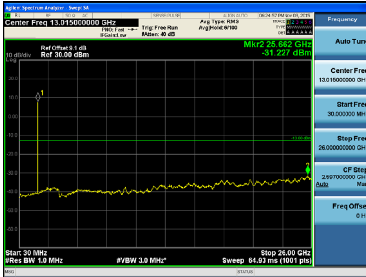
Transmitting Mode, LTE Band IV, MCH(16QAM, Bandwidth=1.4MHz, RB=RB6#0)
