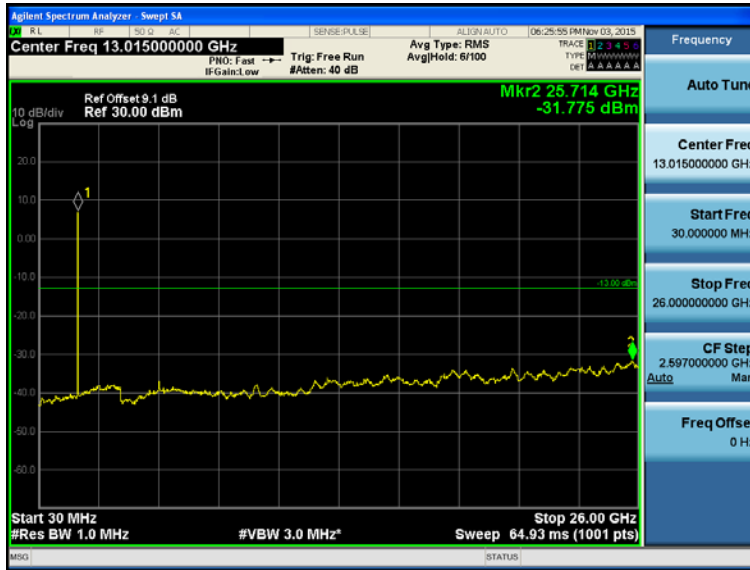
Transmitting Mode, LTE Band IV, LCH(16QAM, Bandwidth=1.4MHz, RB=RB6#0)
