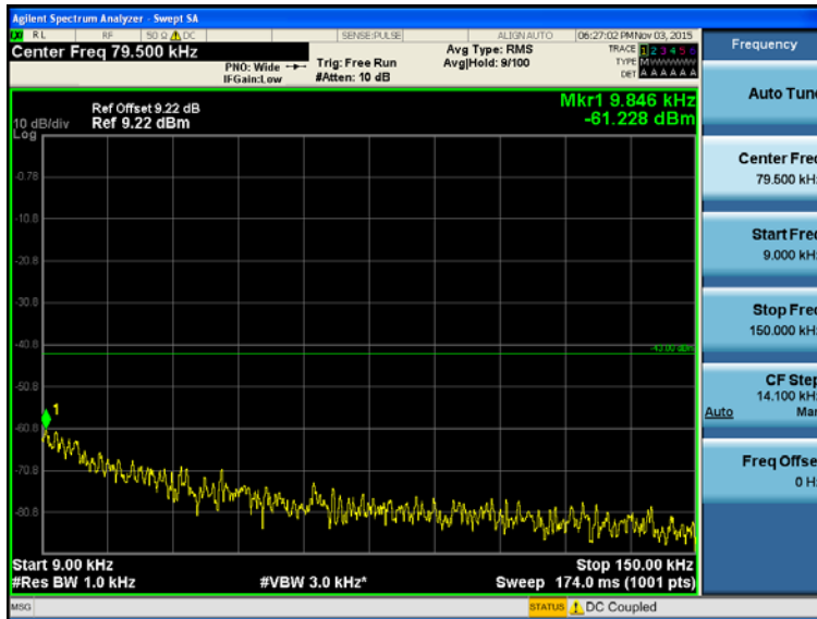
Transmitting Mode, LTE Band IV, MCH(QPSK, Bandwidth=3.0MHz, RB=RB15#0)
