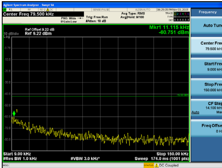
Transmitting Mode, LTE Band IV, MCH(QPSK, Bandwidth=1.4MHz, RB=RB6#0)
