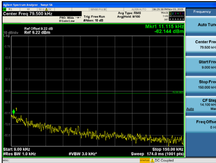
Transmitting Mode, LTE Band IV, HCH(QPSK, Bandwidth=5.0MHz, RB=RB25#0)
