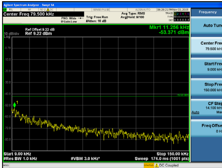
Transmitting Mode, LTE Band IV, LCH(QPSK, Bandwidth=5.0MHz, RB=RB25#0)
