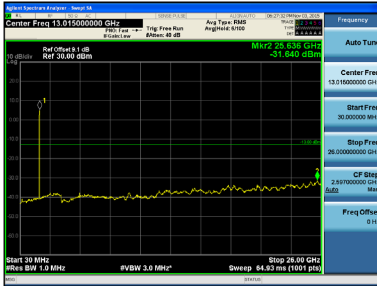
Transmitting Mode, LTE Band IV, HCH(16QAM, Bandwidth=3.0MHz, RB=RB15#0)
