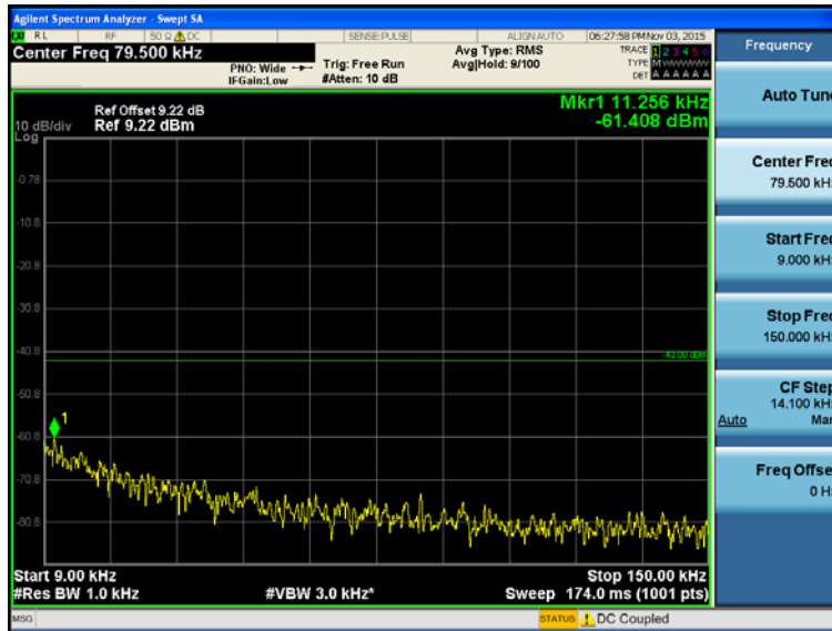
Transmitting Mode, LTE Band IV, HCH(16QAM, Bandwidth=3.0MHz, RB=RB15#0)
