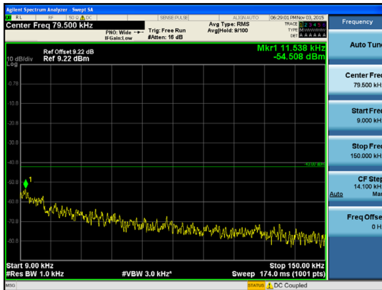
Transmitting Mode, LTE Band IV, MCH(QPSK, Bandwidth=5.0MHz, RB=RB25#0)
