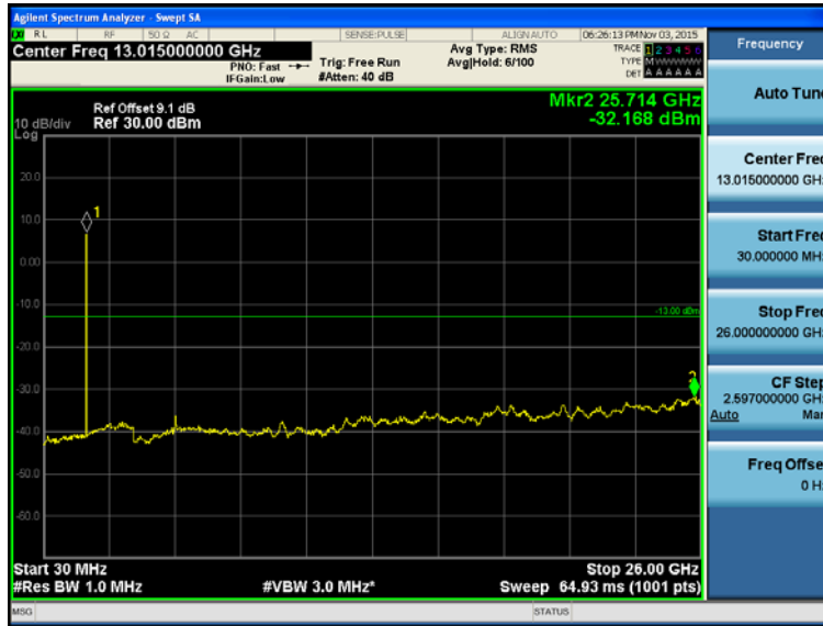
Transmitting Mode, LTE Band IV, LCH(QPSK, Bandwidth=3.0MHz, RB=RB15#0)
