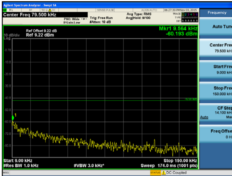
Transmitting Mode, LTE Band IV, HCH(QPSK, Bandwidth=3.0MHz, RB=RB15#0)
