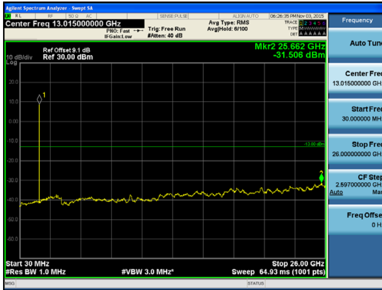
Transmitting Mode, LTE Band IV, MCH(QPSK, Bandwidth=3.0MHz, RB=RB15#0)
