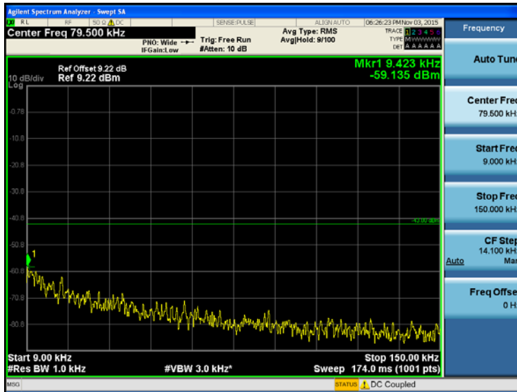
Transmitting Mode, LTE Band IV, LCH(QPSK, Bandwidth=3.0MHz, RB=RB15#0)
