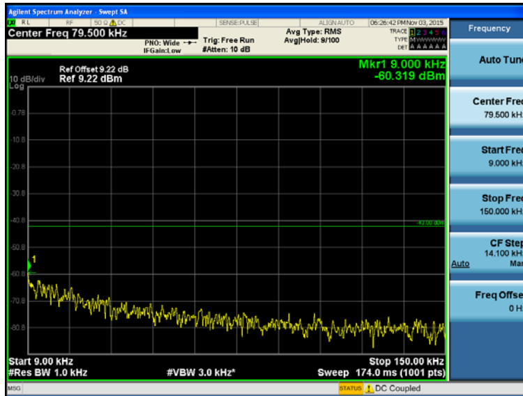
Transmitting Mode, LTE Band IV, LCH(16QAM, Bandwidth=3.0MHz, RB=RB15#0)
