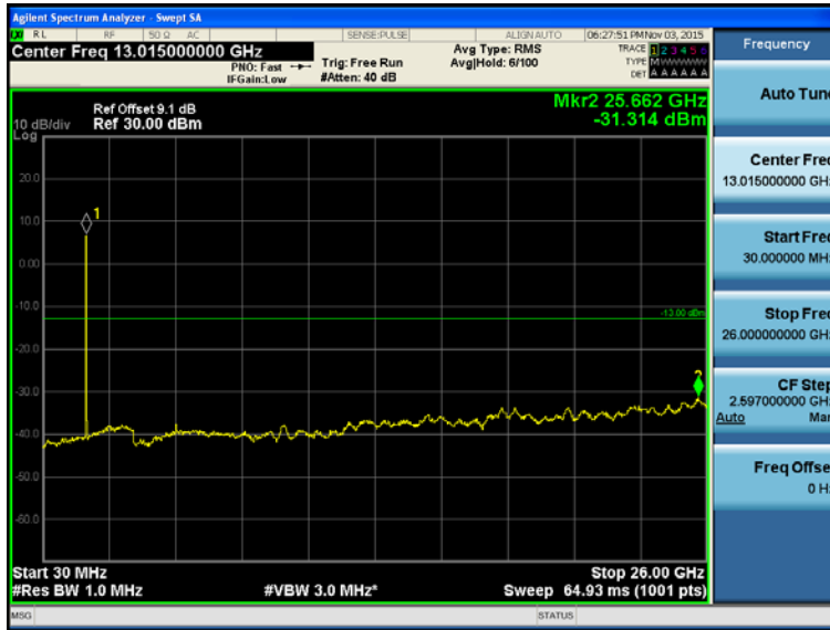
Transmitting Mode, LTE Band IV, LCH(16QAM, Bandwidth=3.0MHz, RB=RB15#0)
