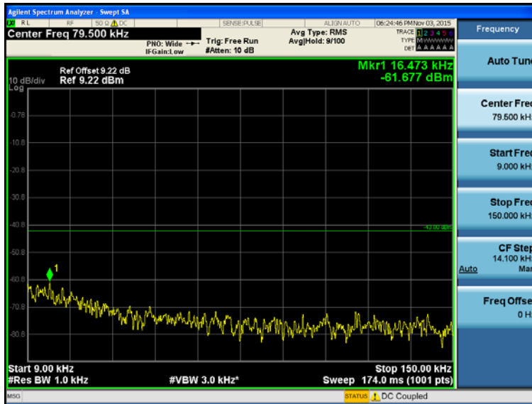
Transmitting Mode, LTE Band IV, LCH(16QAM, Bandwidth=1.4MHz, RB=RB6#0)
