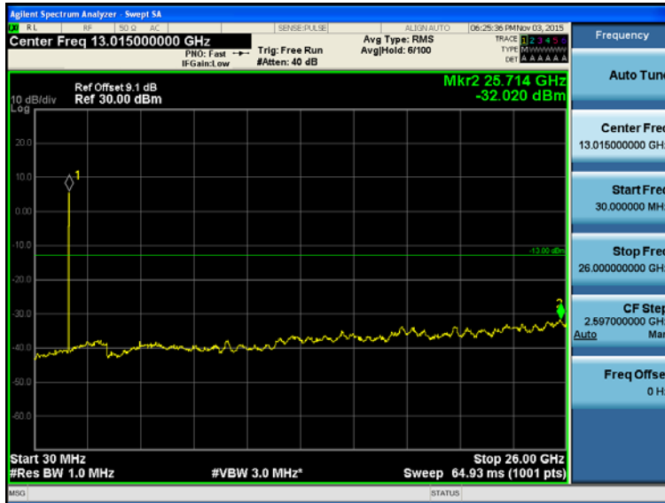
Transmitting Mode, LTE Band IV, HCH(16QAM, Bandwidth=1.4MHz, RB=RB6#0)
