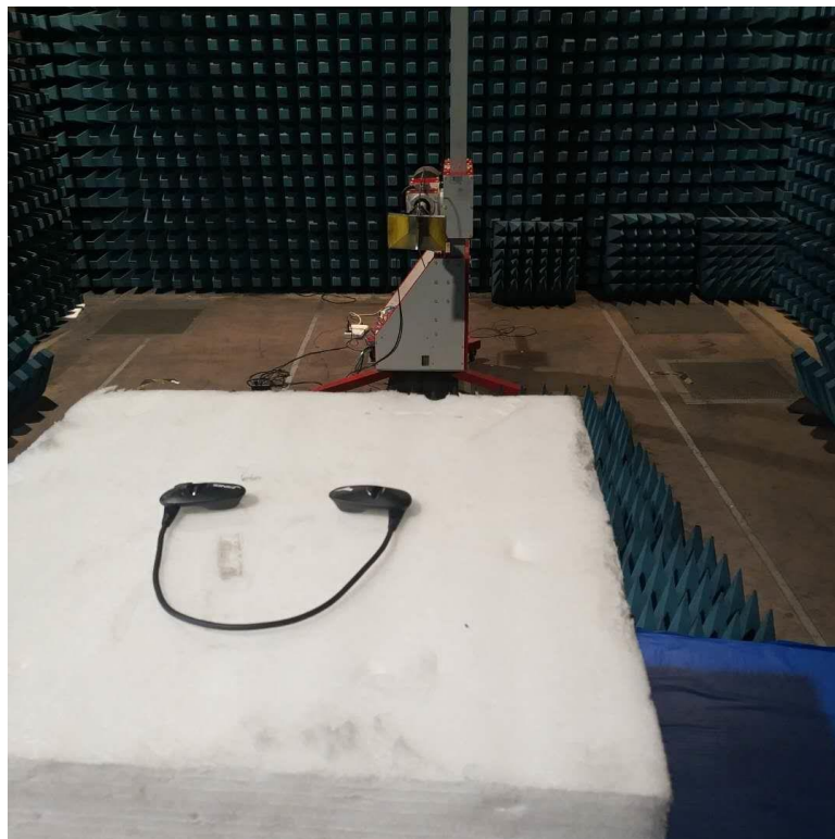
Above 1GHz
