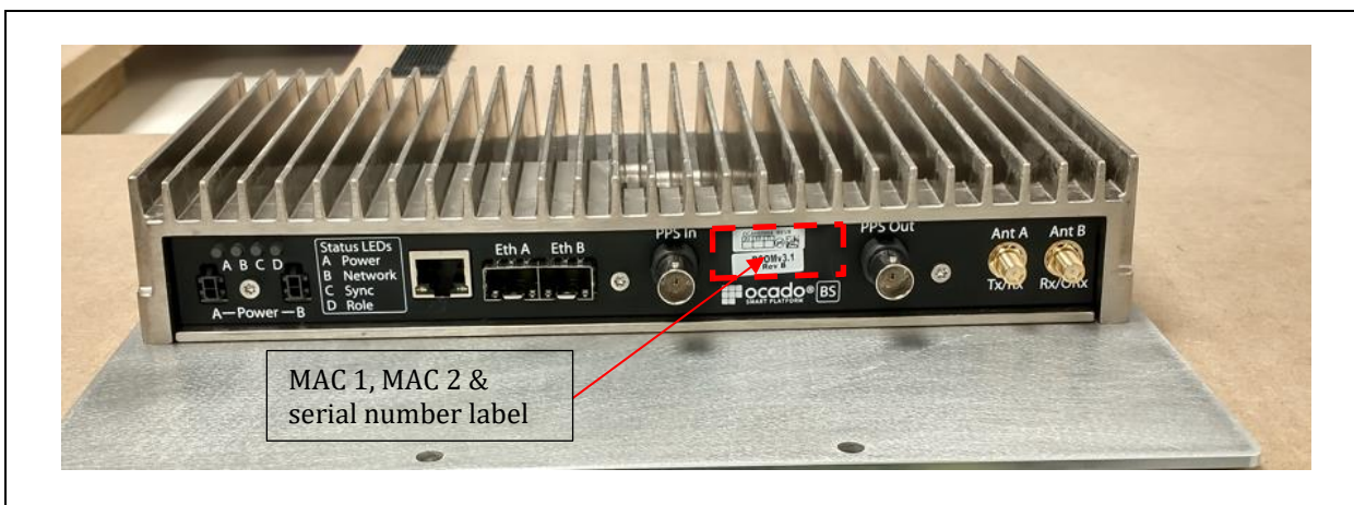
Figure 3 Location for BS MAC 1, MAC 2 & Serial number label
